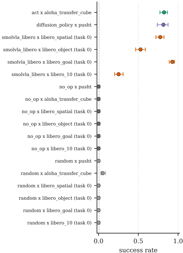
Per-cell success rates - 95% Wilson CI
