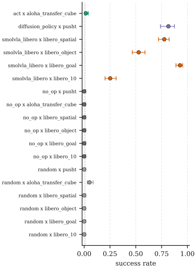
Per-cell success rates - 95% Wilson CI - N=250/cell
