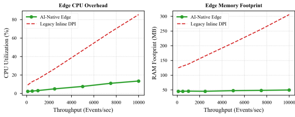
Fig. 4. Edge CPU utilization (%) and RAM footprint (MB) scaling under high throughput (100 to 10,000 events/sec).
