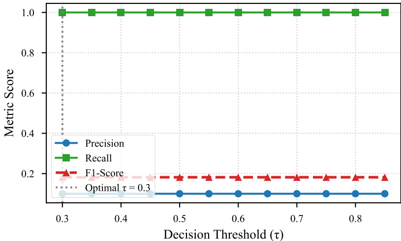
Detection Performance Across Decision Thresholds
