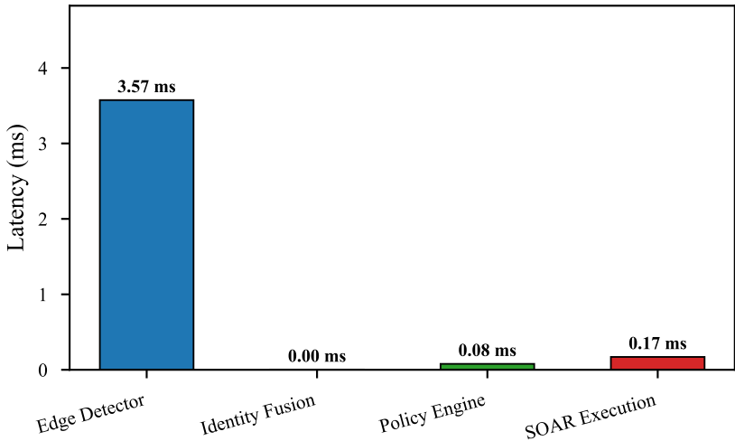
Per-Stage Latency Breakdown (Sub-10ms Pipeline)
