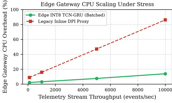
Fig. 5. Edge gateway CPU overhead scaling under high telemetry throughput (100 to 10,000 events/sec).
