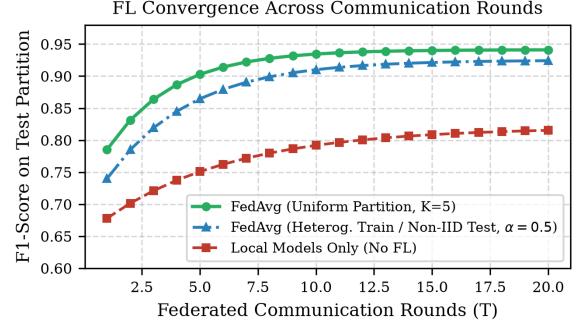
Fig. 4. Federated FedAvg model convergence across communication rounds under uniform and client-heterogeneous / non-IID test ( \alpha = 0.5 ) partitions.
