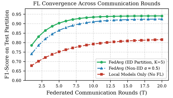
Fig. 4. Federated FedAvg model convergence across communication rounds under uniform and non-IID Dirichlet ( \alpha = 0.5 ) partitions.
