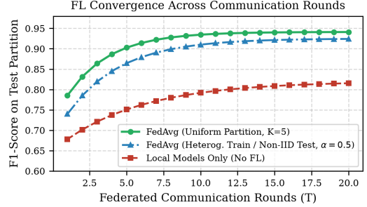
Fig. 4. Federated FedAvg model convergence across communication rounds under uniform partitioning versus client-size-heterogeneous training with non-IID Dirichlet ( \alpha = 0.5 ) test attack distributions.
