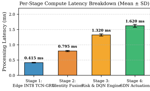
Fig. 2. Per-stage compute latency breakdown (Mean \pm SD ms) across 1,000 flow trials.
