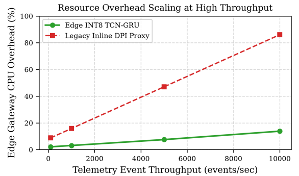
Fig. 4. Edge CPU utilization (%) scaling under high throughput (100 to 10,000 events/sec).
