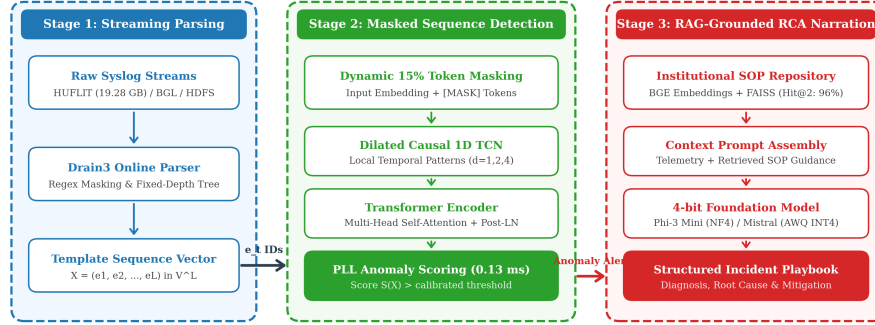
Fig. 1. Architectural Overview of the LLM-Augmented AIOps Framework: (1) Streaming Drain3 log parsing and template encoding; (2) Masked TCN-Transformer autoencoder sequence scoring; and (3) RAG-Grounded Quantized Foundation Model Root Cause Narration Engine.
