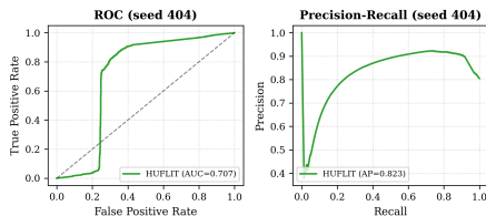
Fig. 2. Protocol A ROC/PR for seed 404 (illustrative; first of the five evaluation seeds in tables; mean \pm std reported separately).
