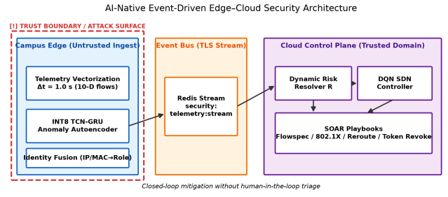
Fig. 1. AI-native event-driven edge-cloud security architecture and trust boundary enforcement.
