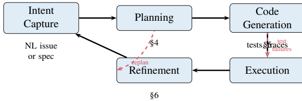
Figure 1 The vibe coding pipeline. Intent flows through planning, generation, and execution. Test failures trigger refinement; replanning occurs when the initial hypothesis is invalidated. Section 3 surveys full-pipeline systems; subsequent sections zoom into individual stages.
