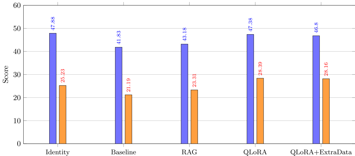
Qwen3.5-2B: SARI and BI ■ SARI ■ BLEU paraphrase test split (N=667)
