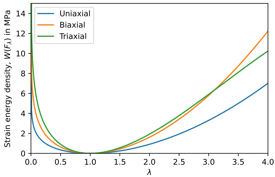
Figure 3.1: The variation of the Neo-Hookean energy density as a function of various forms of stretch. Here, a=0.6\text{MPa} and c=0.6\text{MPa} , which are values representative of rubber.
