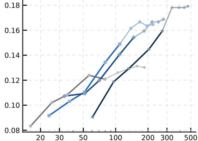
MATH500
