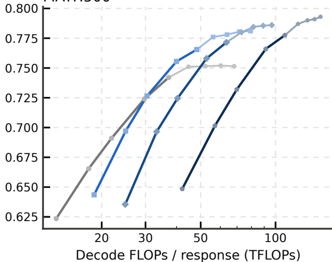
MATH500
