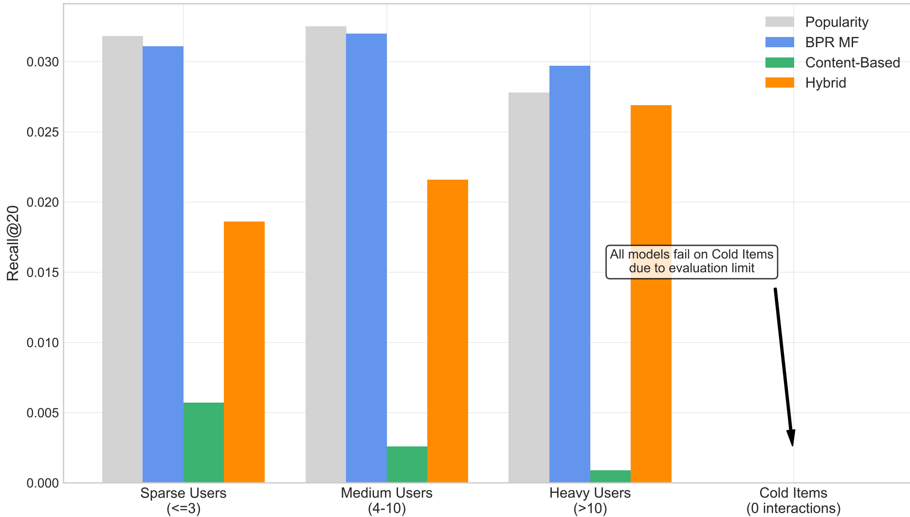
Model Performance across User and Item Slices
