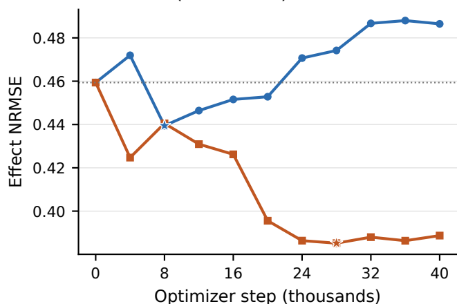
Seed B (cross-seed) · Effect NRMSE
