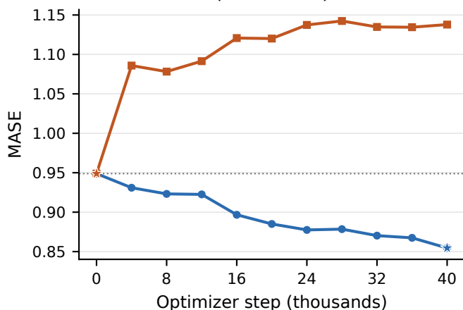
Seed B (cross-seed) · MASE
