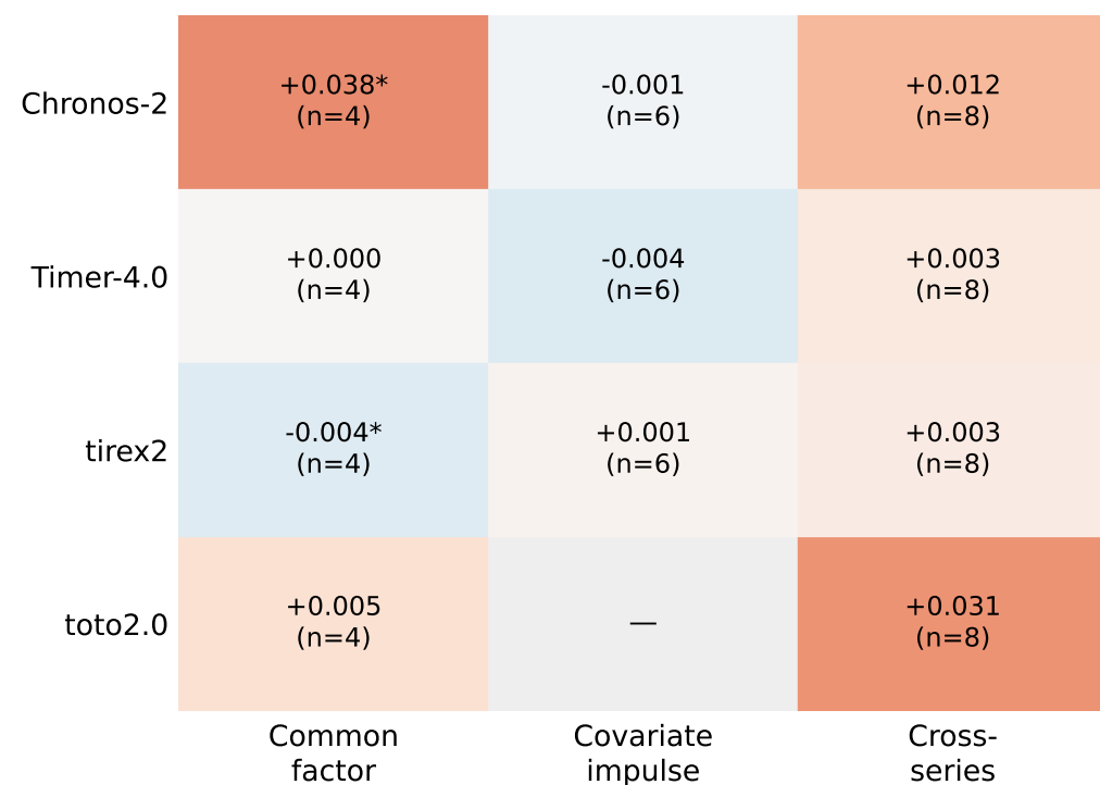
GIFT-Long
