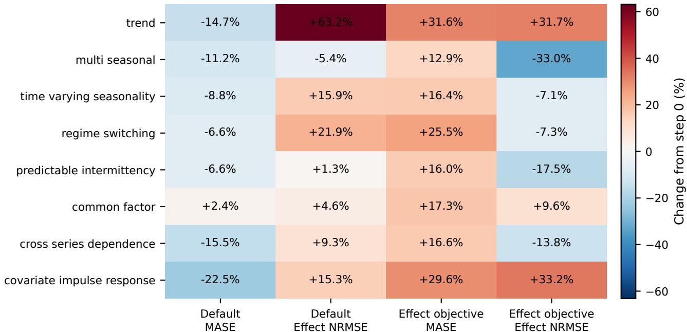
Seed B capability-wise change at 40k steps (lower is better)
