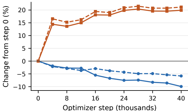
Macro-stratum MASE
