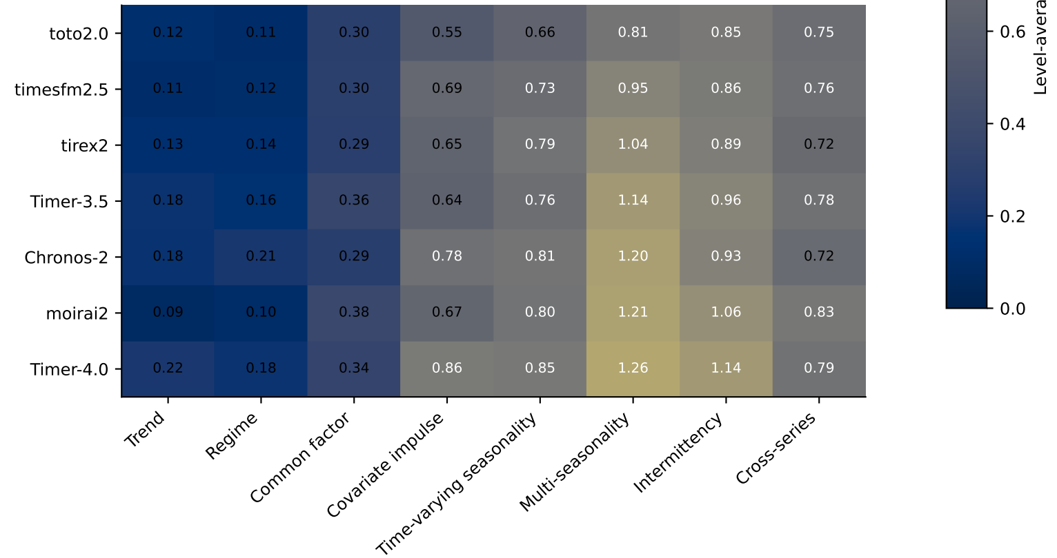
FEV-Mini20 (models ordered by derived macro)
