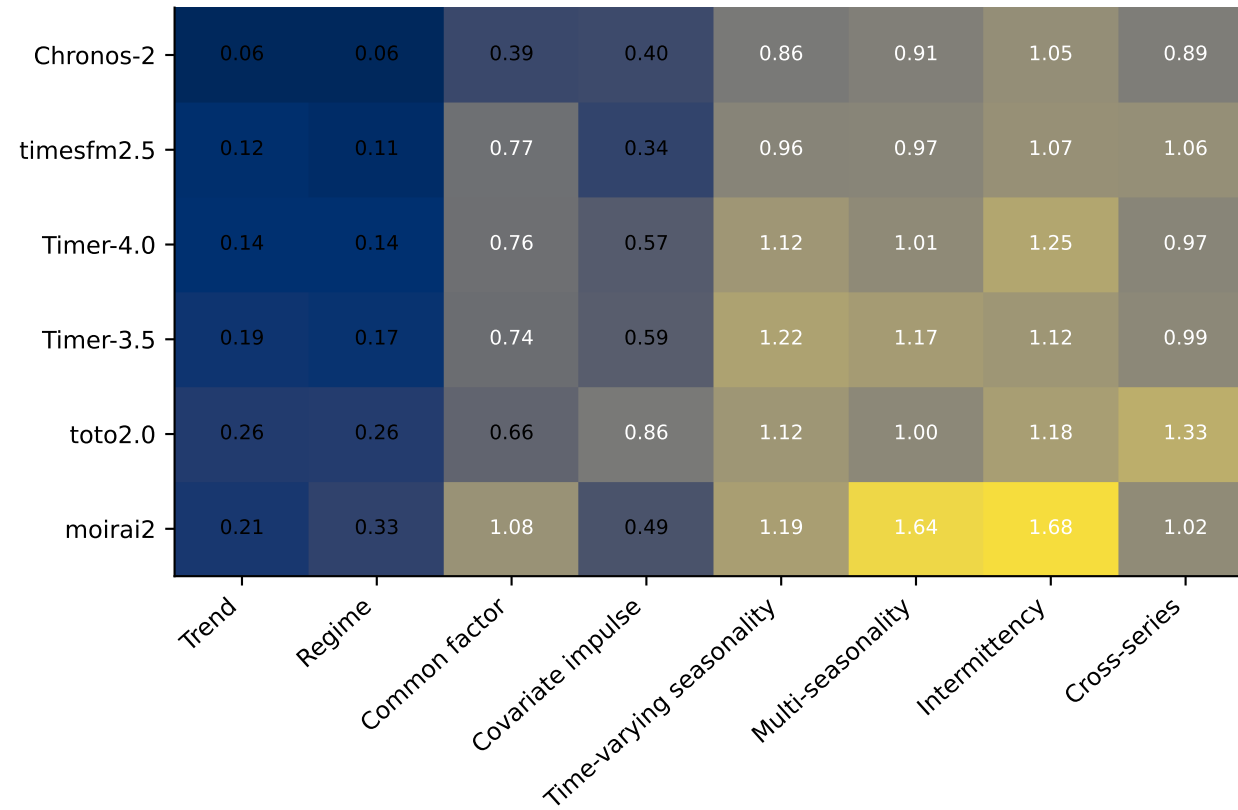
GIFT-Long (models ordered by derived macro)
