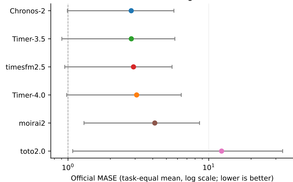
GIFT-Long
