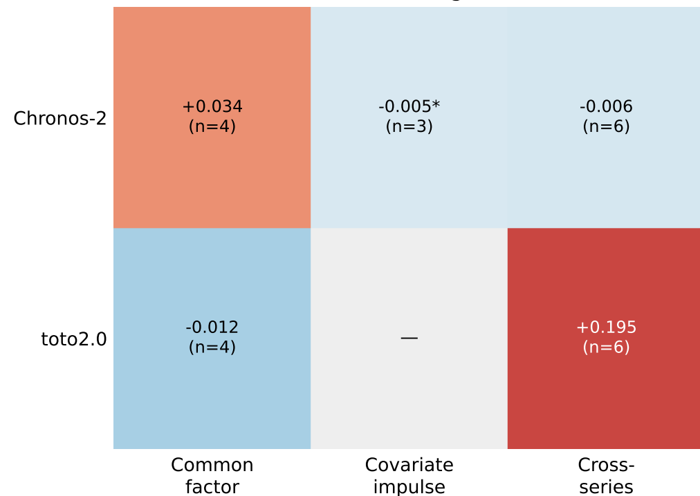
GIFT-Long
