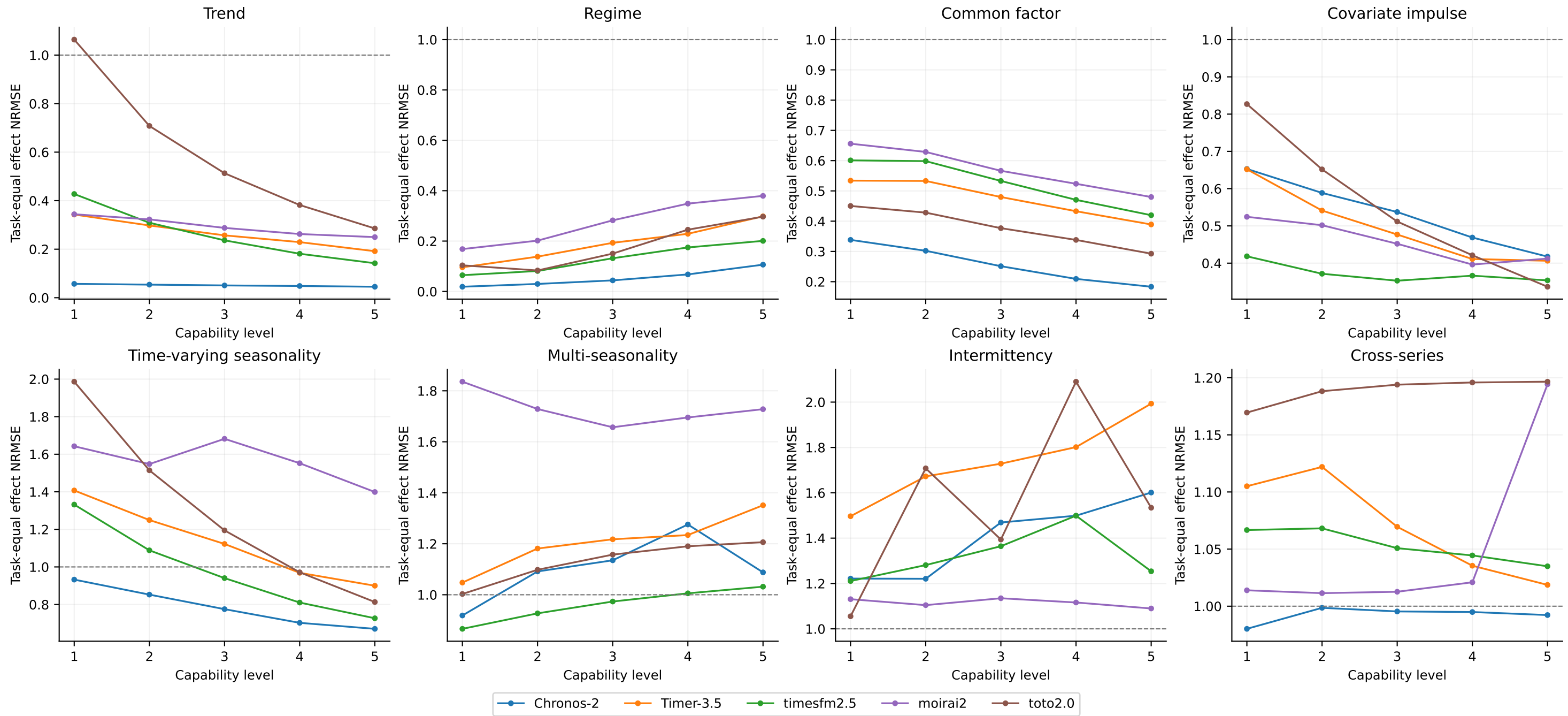
GIFT-Medium: capability response across levels (NRMSE=1 is zero-response reference)
