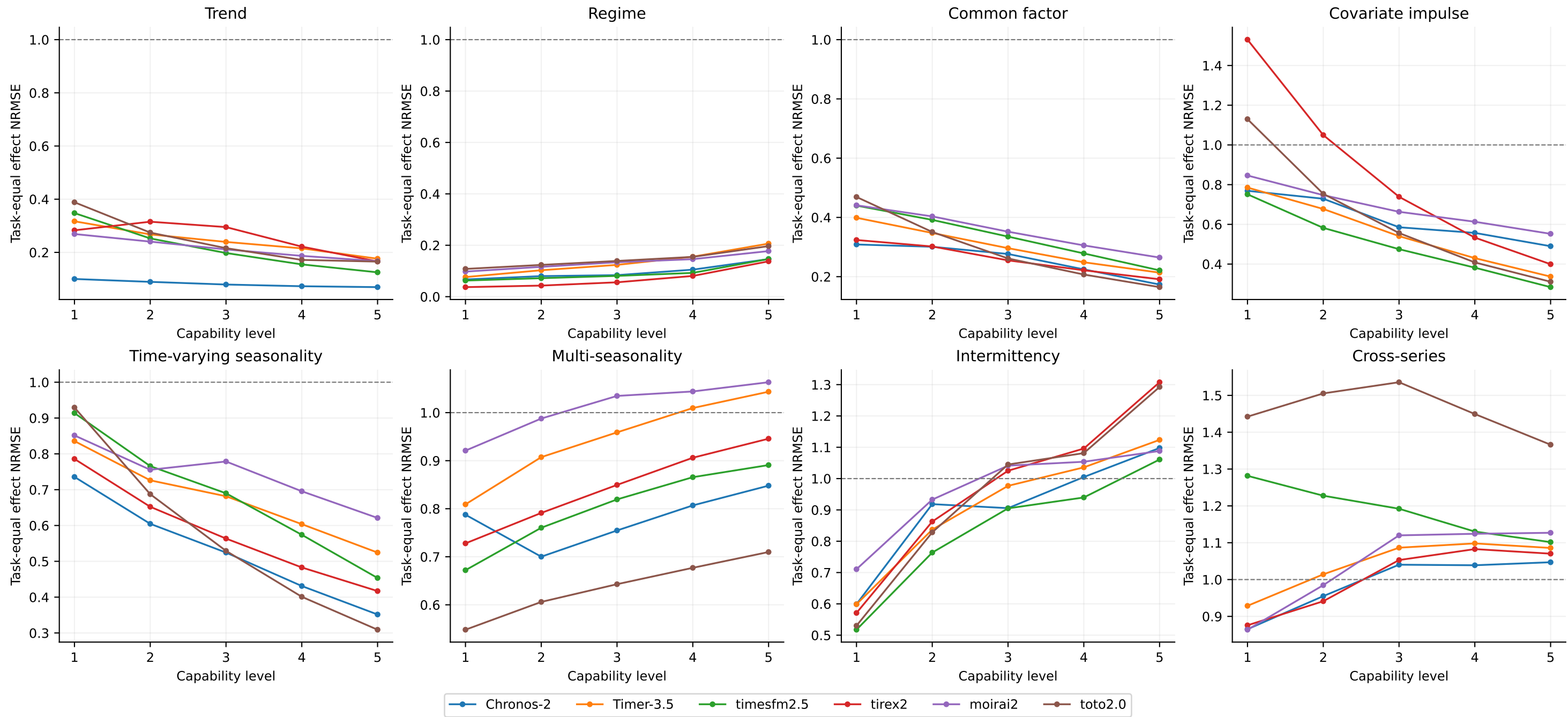
GIFT-Short: capability response across levels (NRMSE=1 is zero-response reference)
