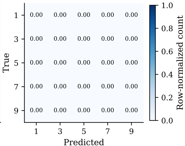
iTransformer
