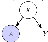
OBSERVED_CONFOUNDER (no A \rightarrow Y )
