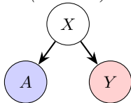
OBSERVED_CONFOUNDER (no A \rightarrow Y )
