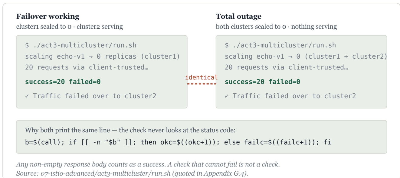
Figure 11.3 — One check, two opposite realities, the same output.
