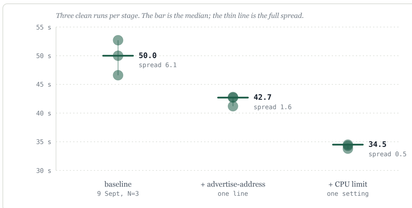
Figure 8.1 — Two one-line changes: the median falls from 50.0 s to 34.5 s, and the spread from 6.1 s to 0.5 s.
