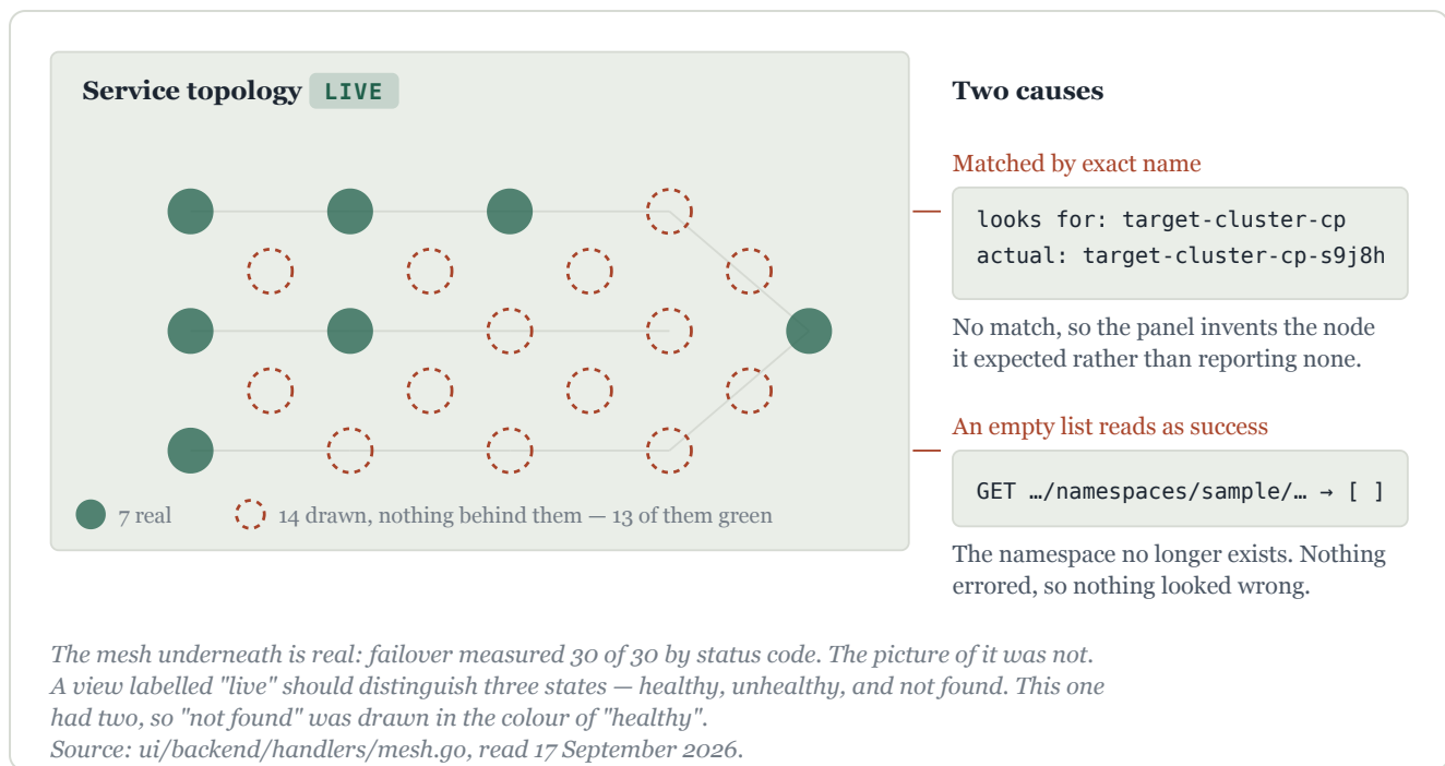
Figure 12.2 — A view labelled "live", drawing fourteen things that do not exist.
