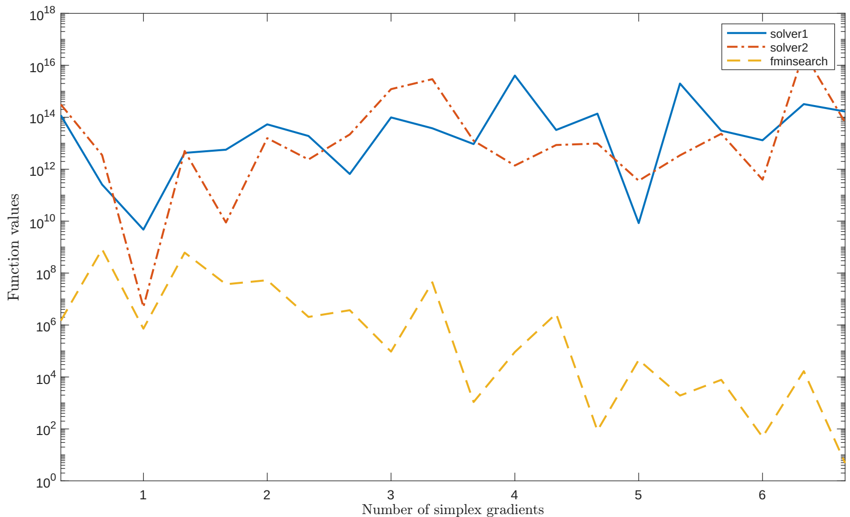
Solving "MEXHAT" with "noisy_0.001_mixed_gaussian" feature
