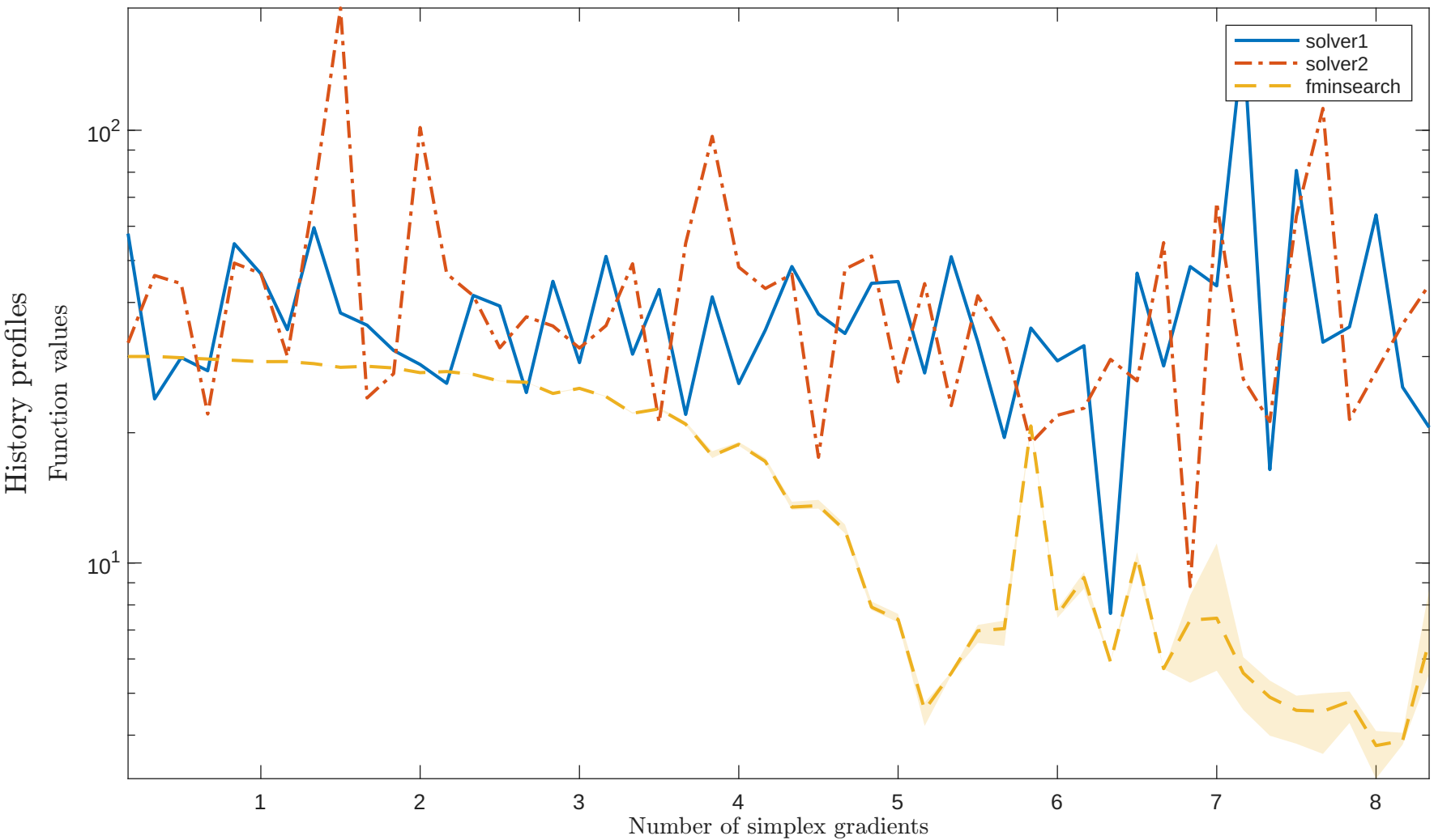
Solving “QING” with “noisy_0.001_mixed_gaussian” feature
