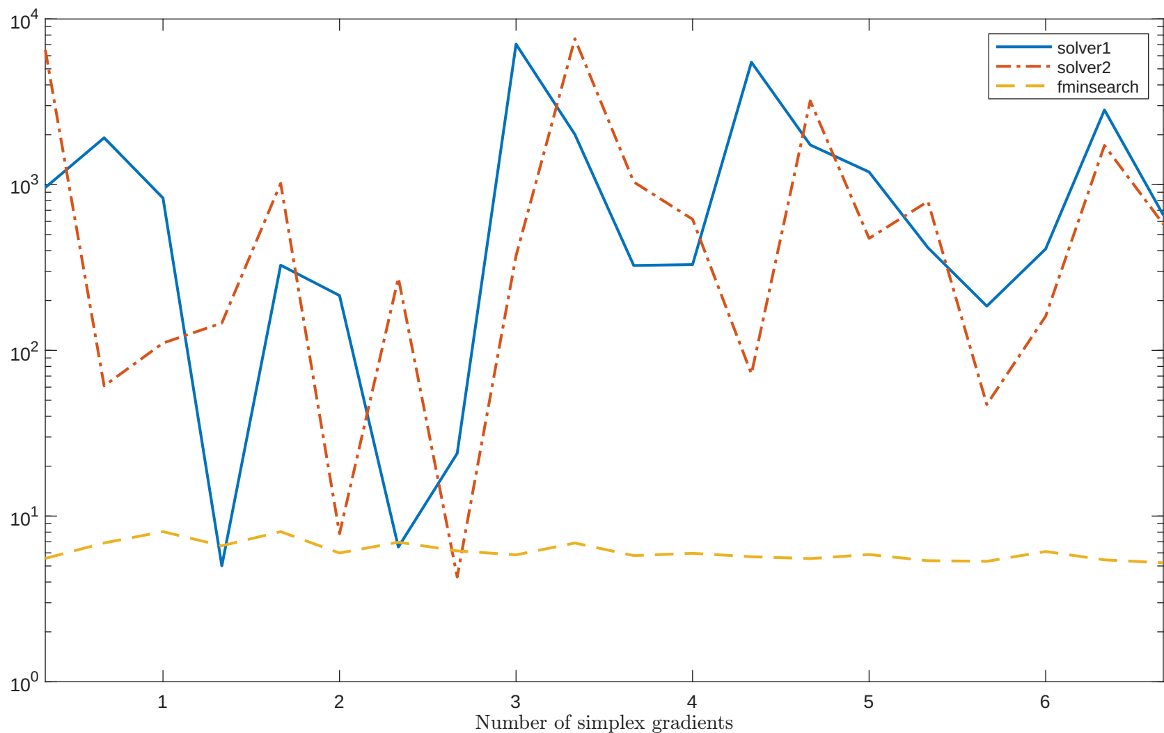
Solving "SINEVAL" with "noisy_0.001_mixed_gaussian" feature
