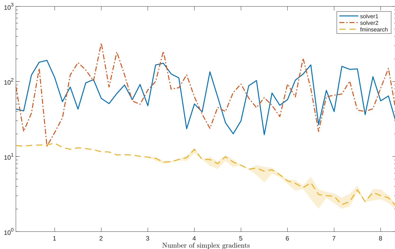
Solving "TRIDIA" with "noisy_0.001_mixed_gaussian" feature
