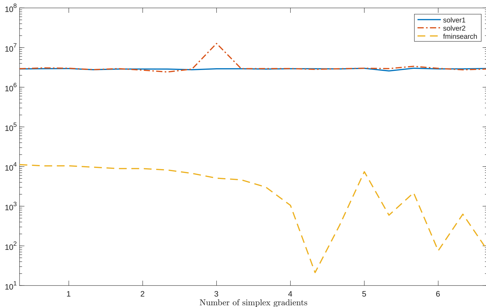
Solving "MISRA1DLS" with "noisy_0.001_mixed_gaussian" feature
