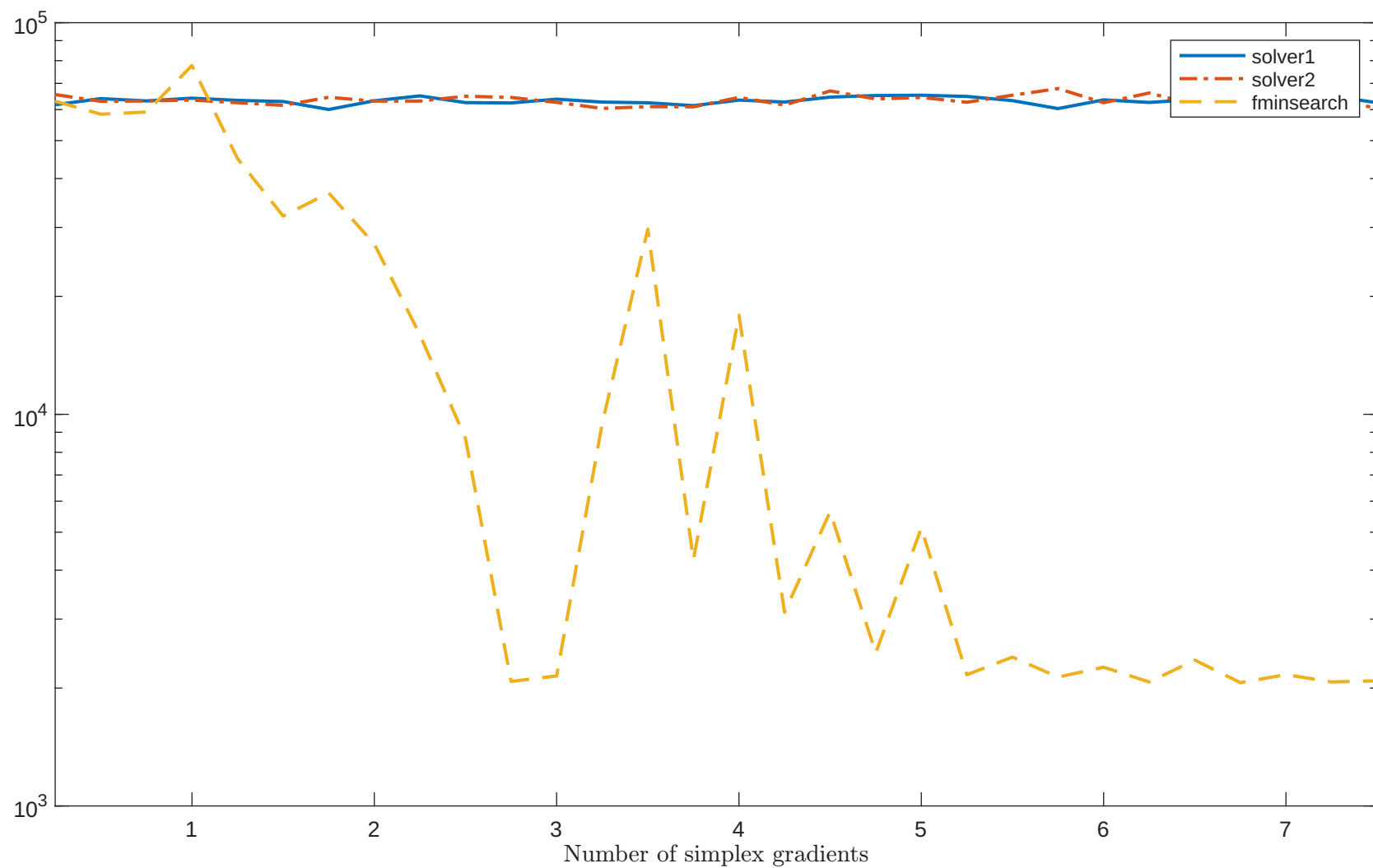
Solving "LSC1LS" with "noisy_0.001_mixed_gaussian" feature
