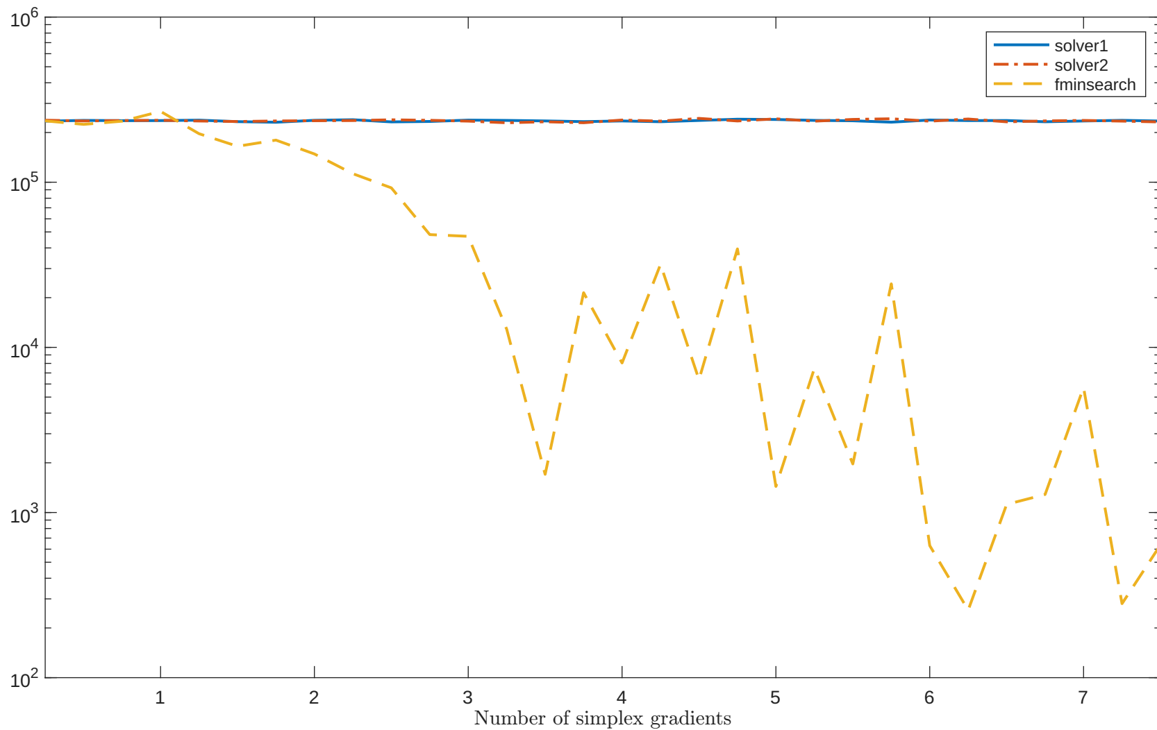
Solving "LSC2LS" with "noisy_0.001_mixed_gaussian" feature
