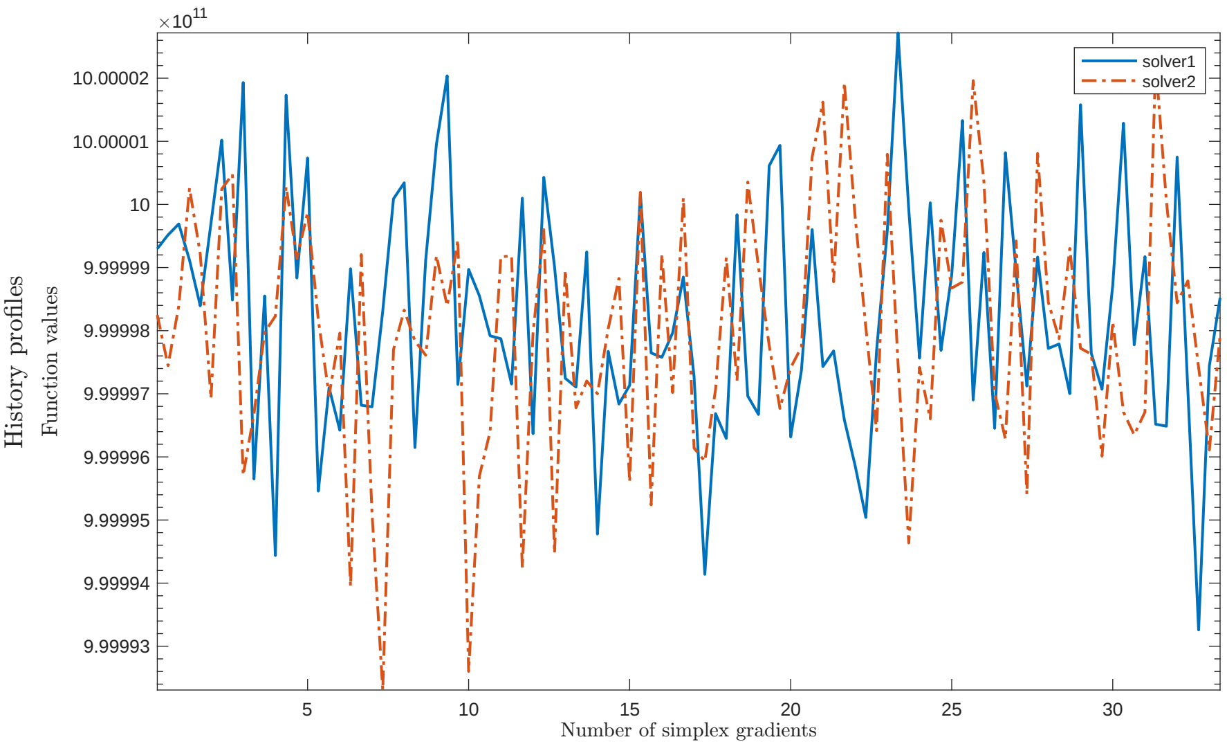
Solving "BROWNBS" with "plain" feature
