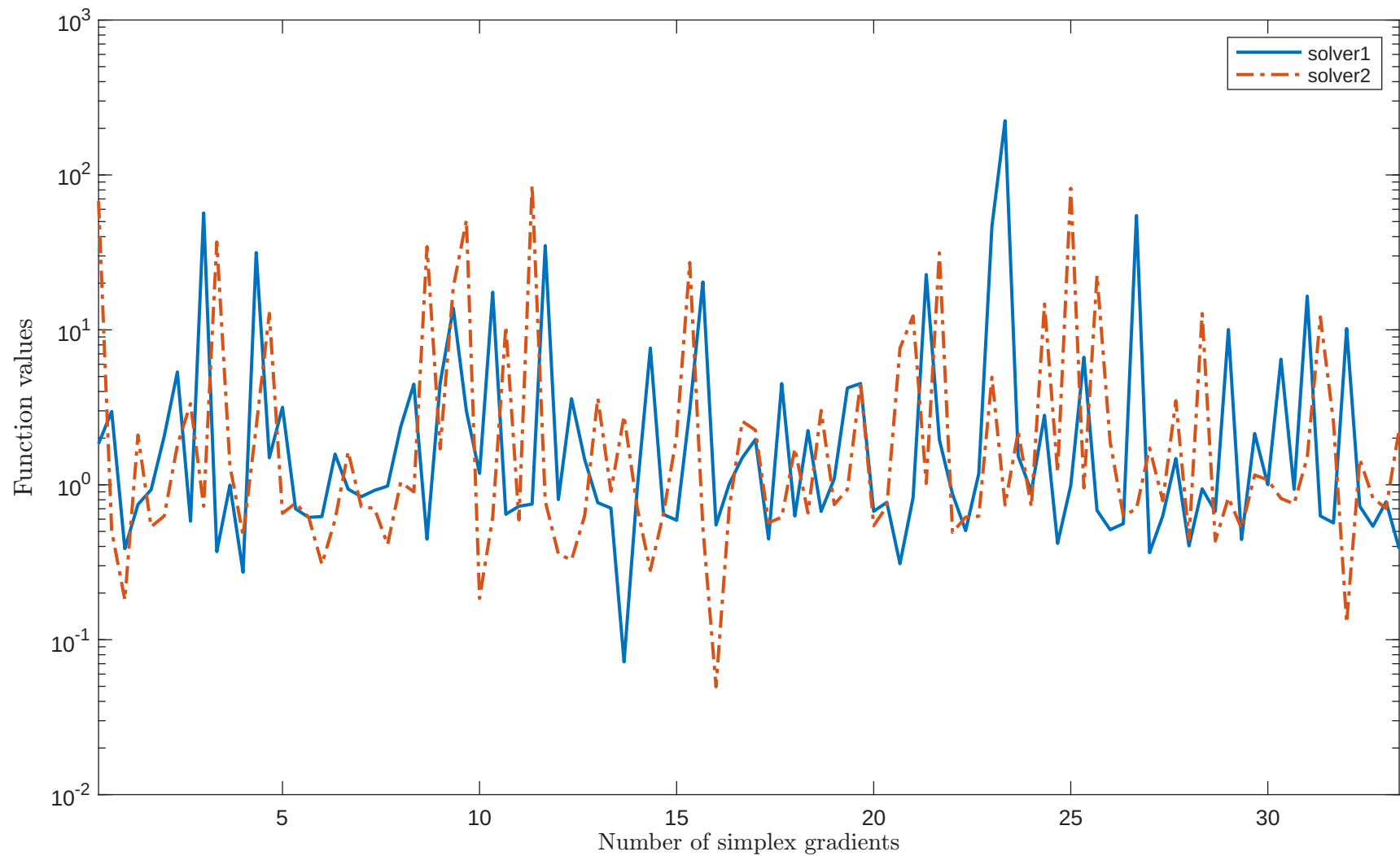
Solving "HIMMELBG" with "plain" feature
