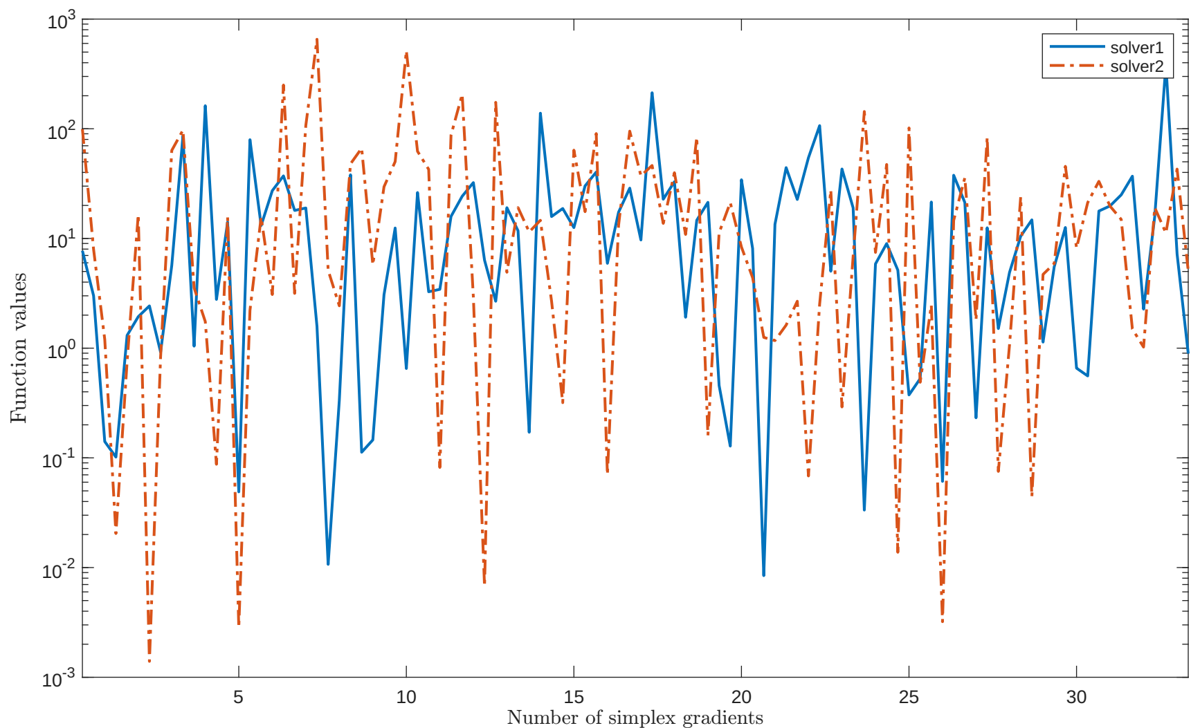
Solving "SISSER2" with "plain" feature
