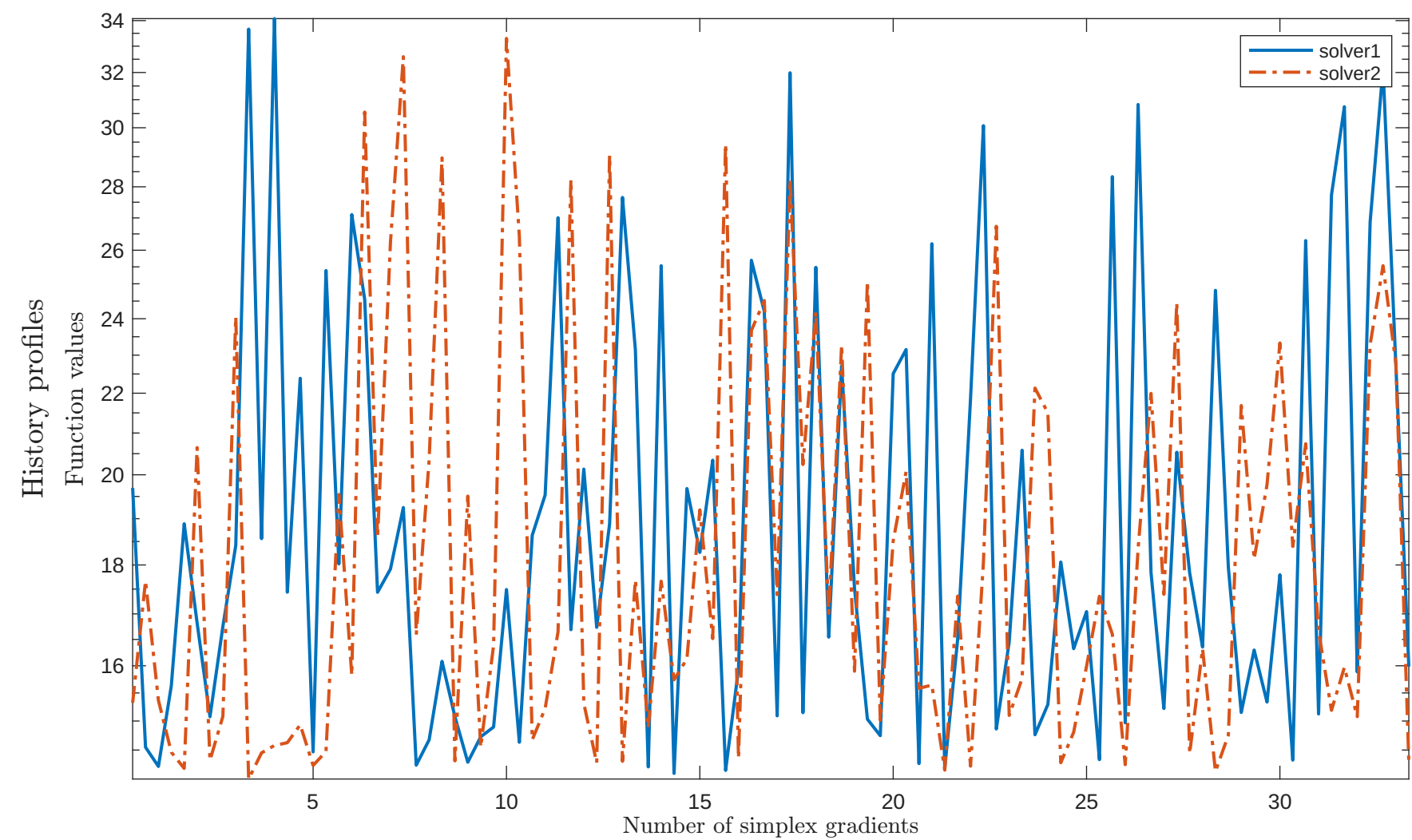
Solving "SNAIL" with "plain" feature
