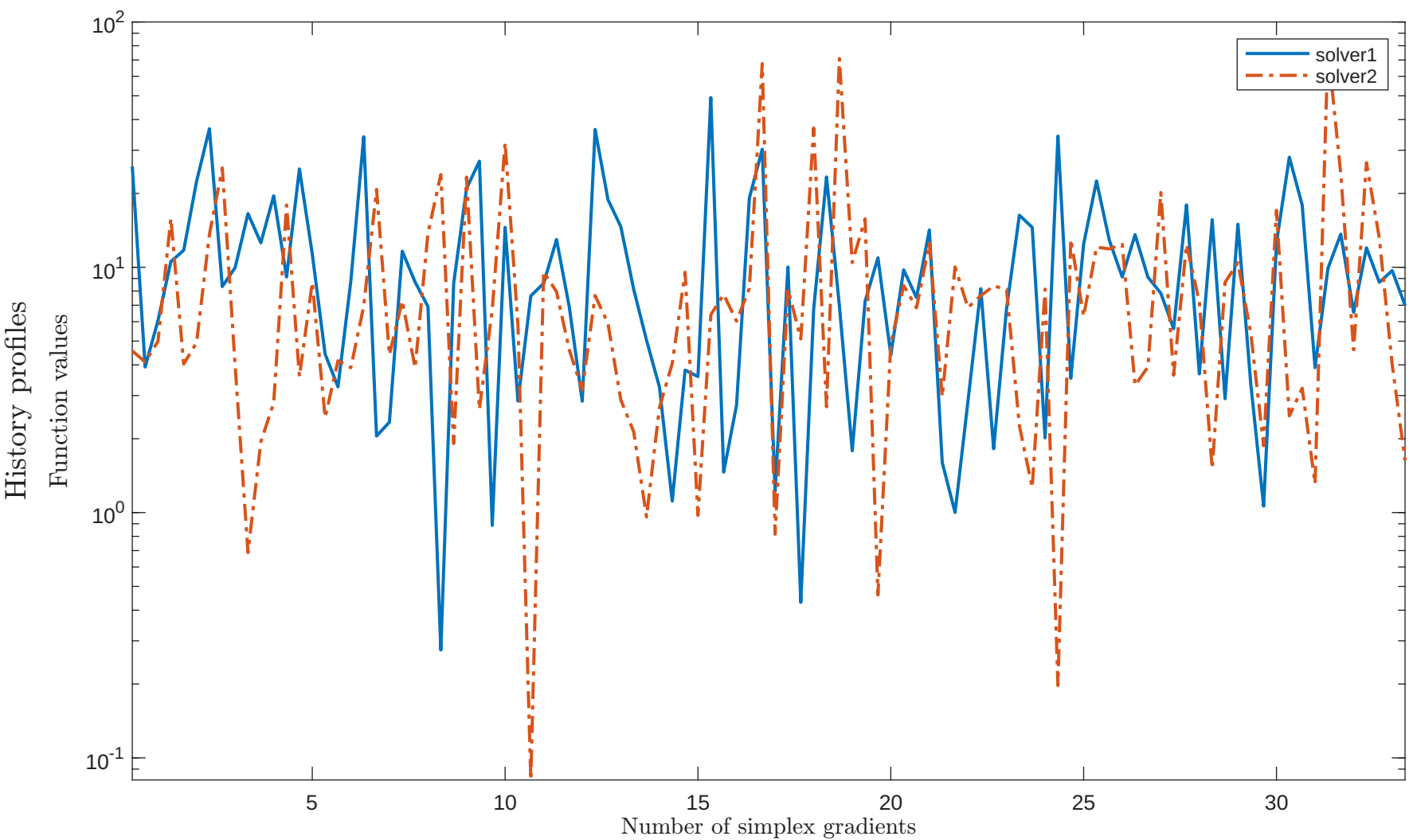
Solving "DENSCHNB" with "plain" feature
