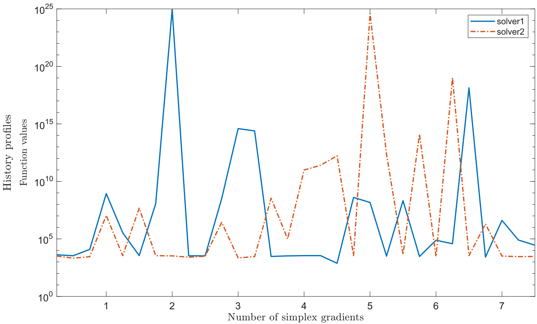
Solving “GROWTHLS” with “noisy_0.001_mixed_gaussian” feature
