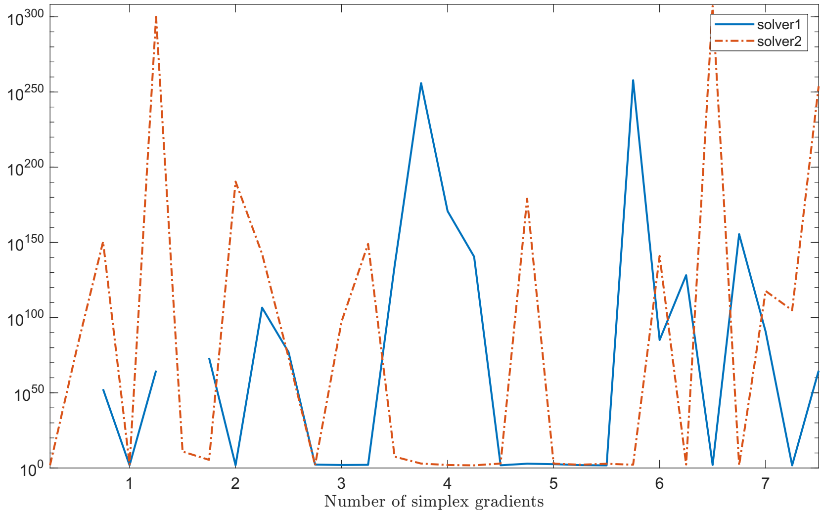
Solving “NELSONLS” with “noisy_0.001_mixed_gaussian” feature
