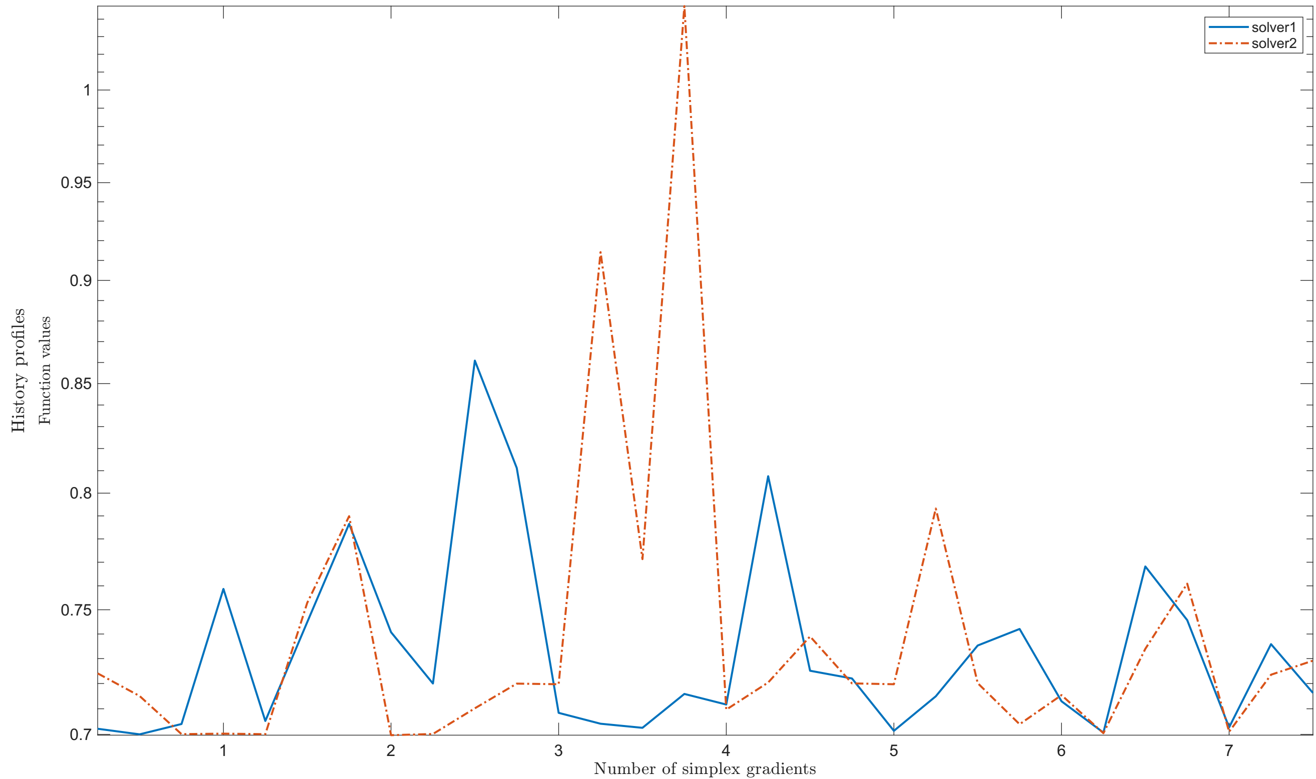
Solving “ECKERLE4LS” with “noisy_0.001_mixed_gaussian” feature
