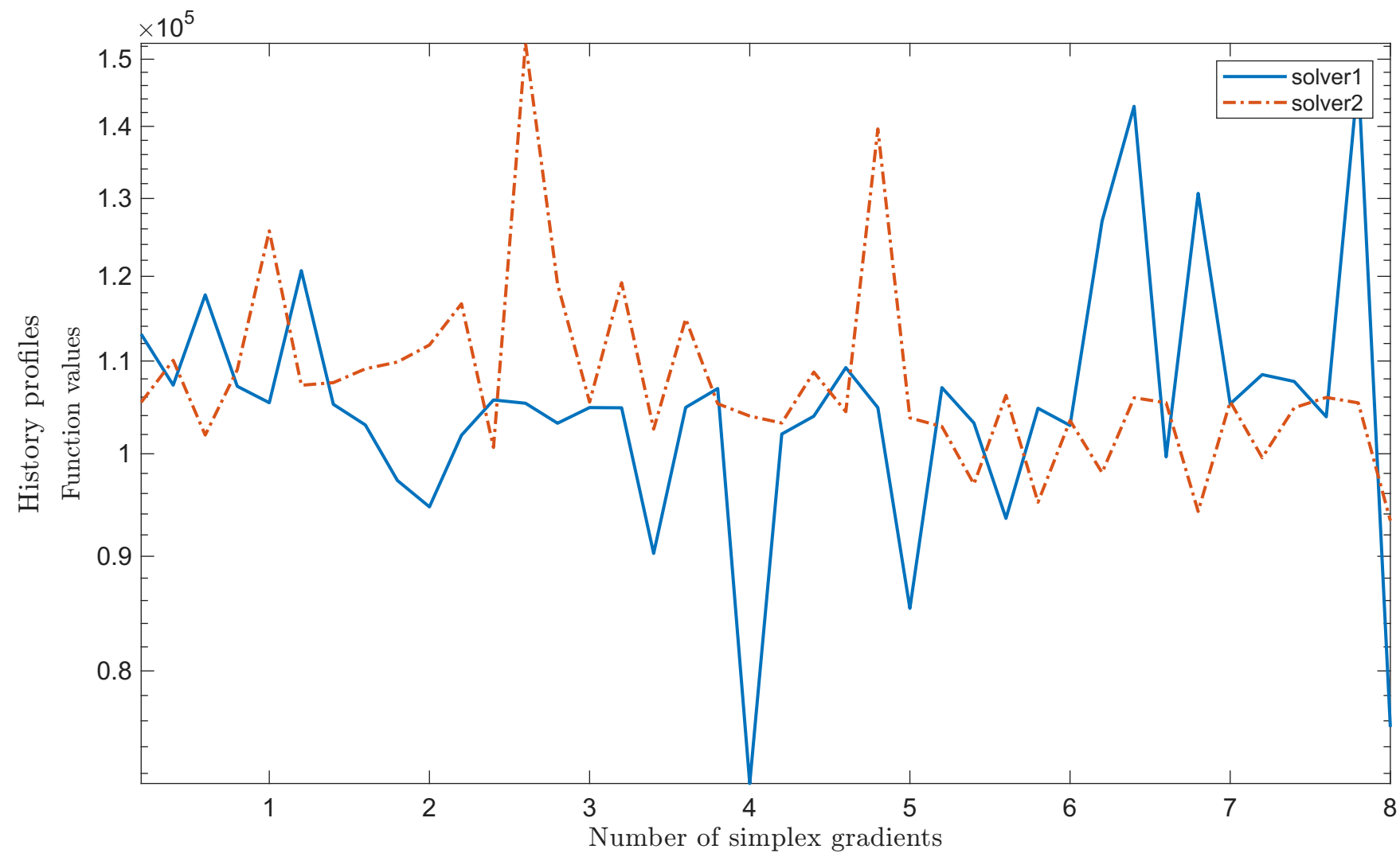
Solving “DEVGLA1” with “noisy_0.001_mixed_gaussian” feature
