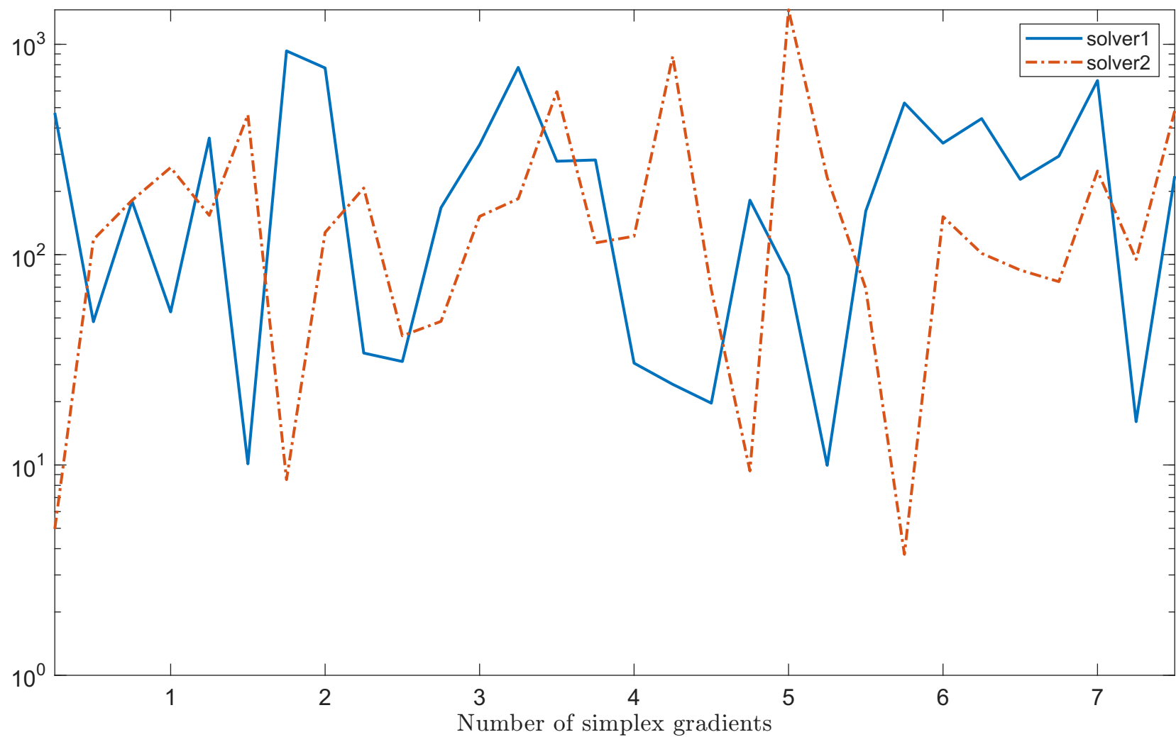
Solving "DENSCHNE" with "noisy_0.001_mixed_gaussian" feature
