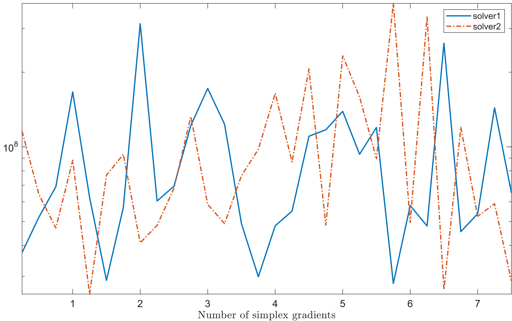
Solving "DENSCHND" with "noisy_0.001_mixed_gaussian" feature
