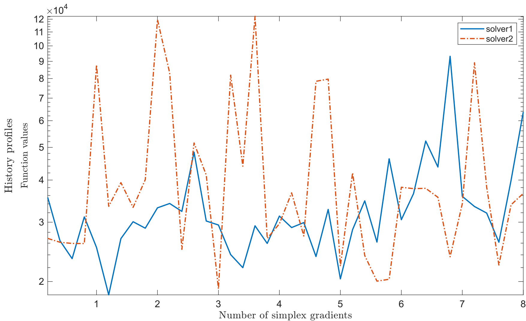
Solving "HIMMELBF" with "noisy_0.001_mixed_gaussian" feature
