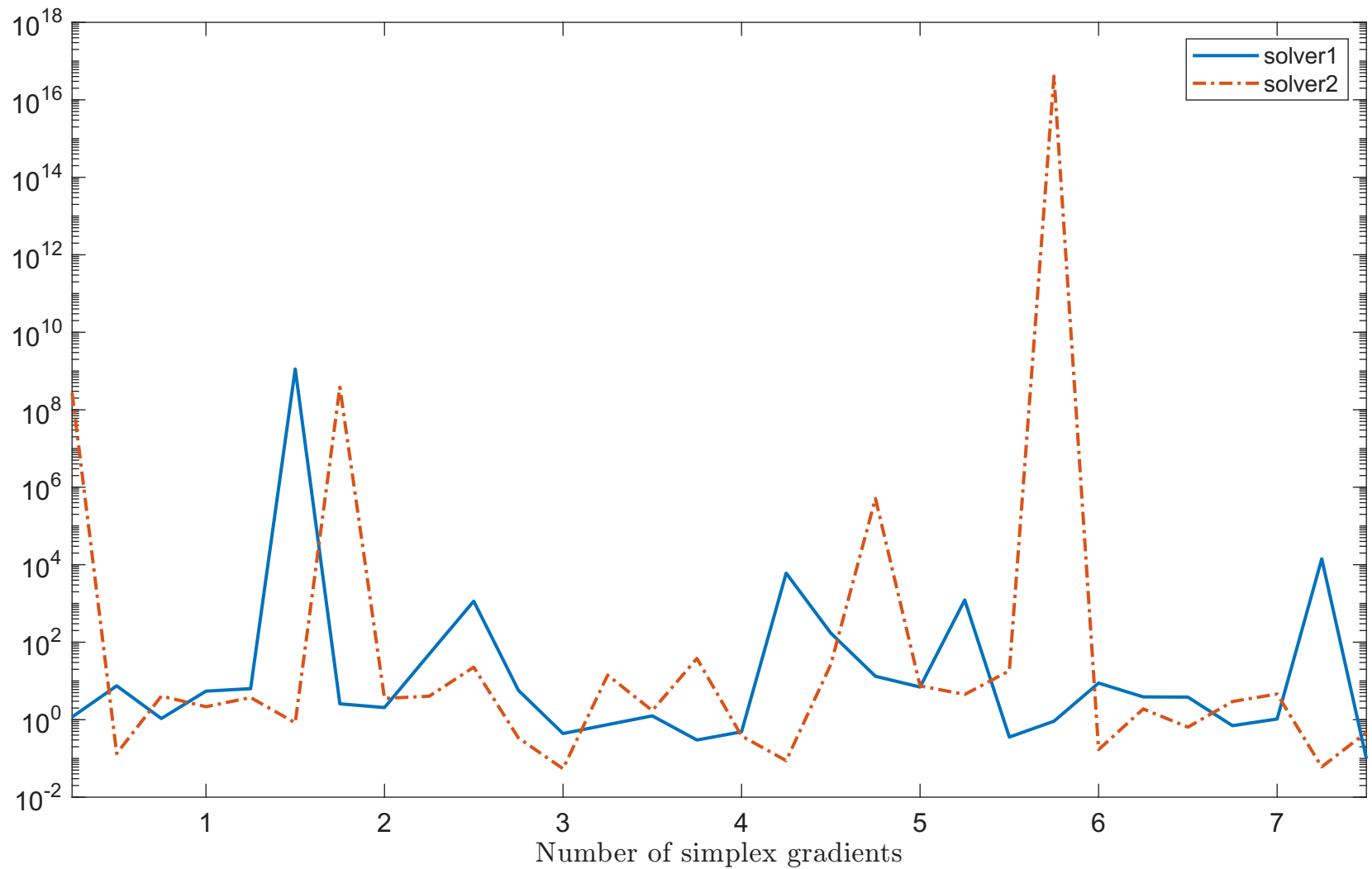
Solving “GAUSSIAN” with “noisy_0.001_mixed_gaussian” feature
