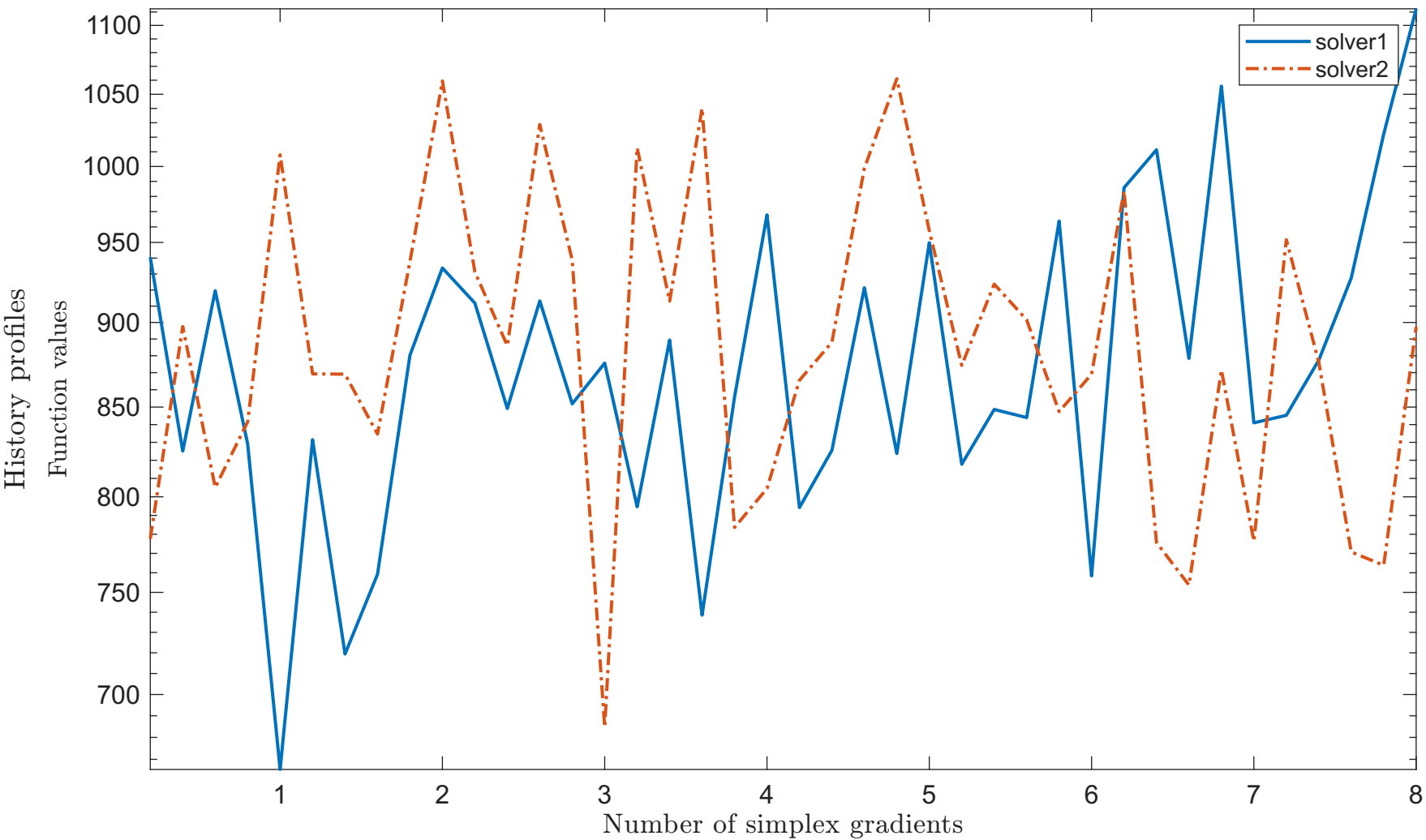
Solving “MGH09LS” with “noisy_0.001_mixed_gaussian” feature
