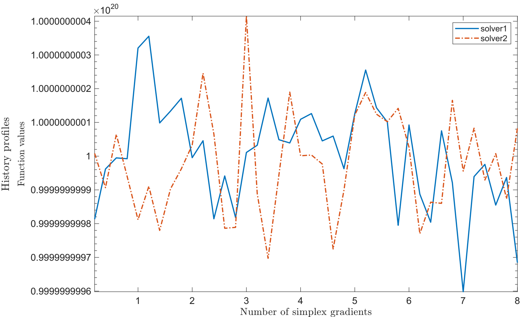
Solving “STREG” with “noisy_0.001_mixed_gaussian” feature
