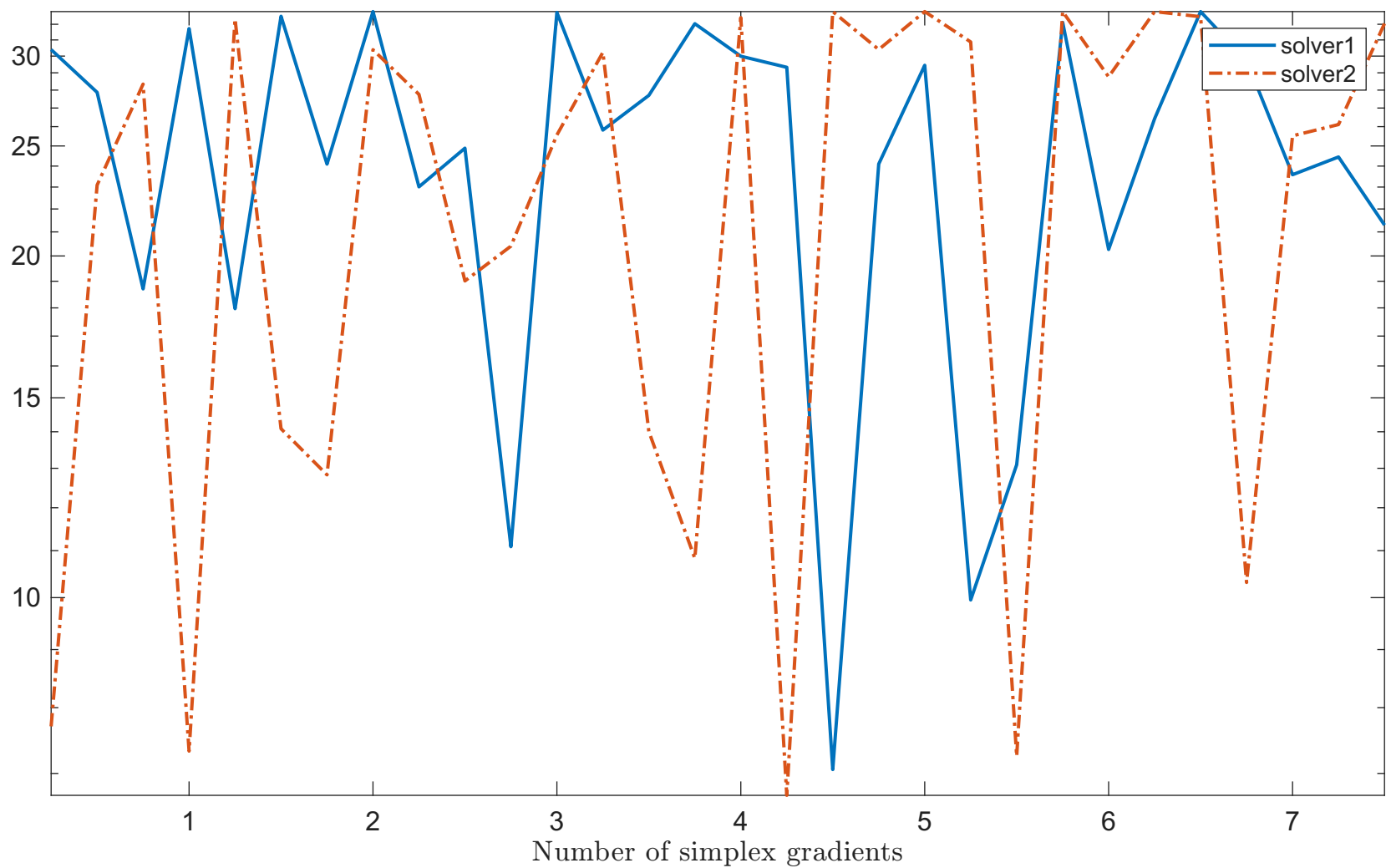
Solving "GULF" with "noisy_0.001_mixed_gaussian" feature
