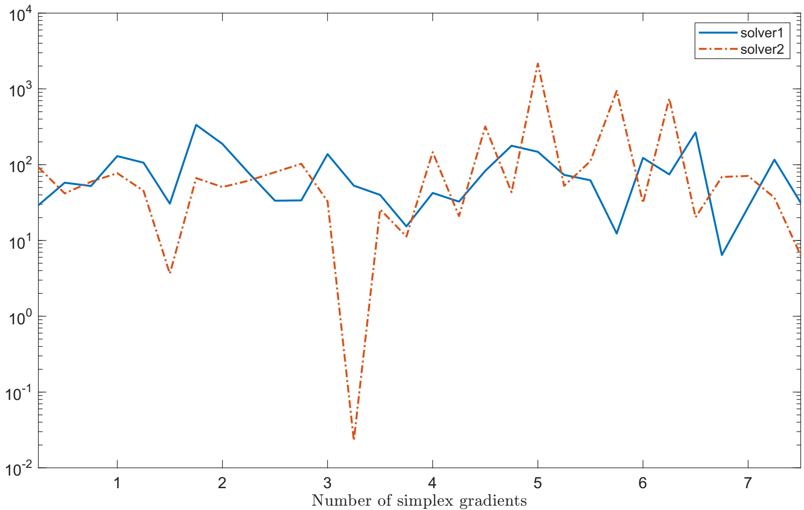
Solving “HATFLDE” with “noisy_0.001_mixed_gaussian” feature
