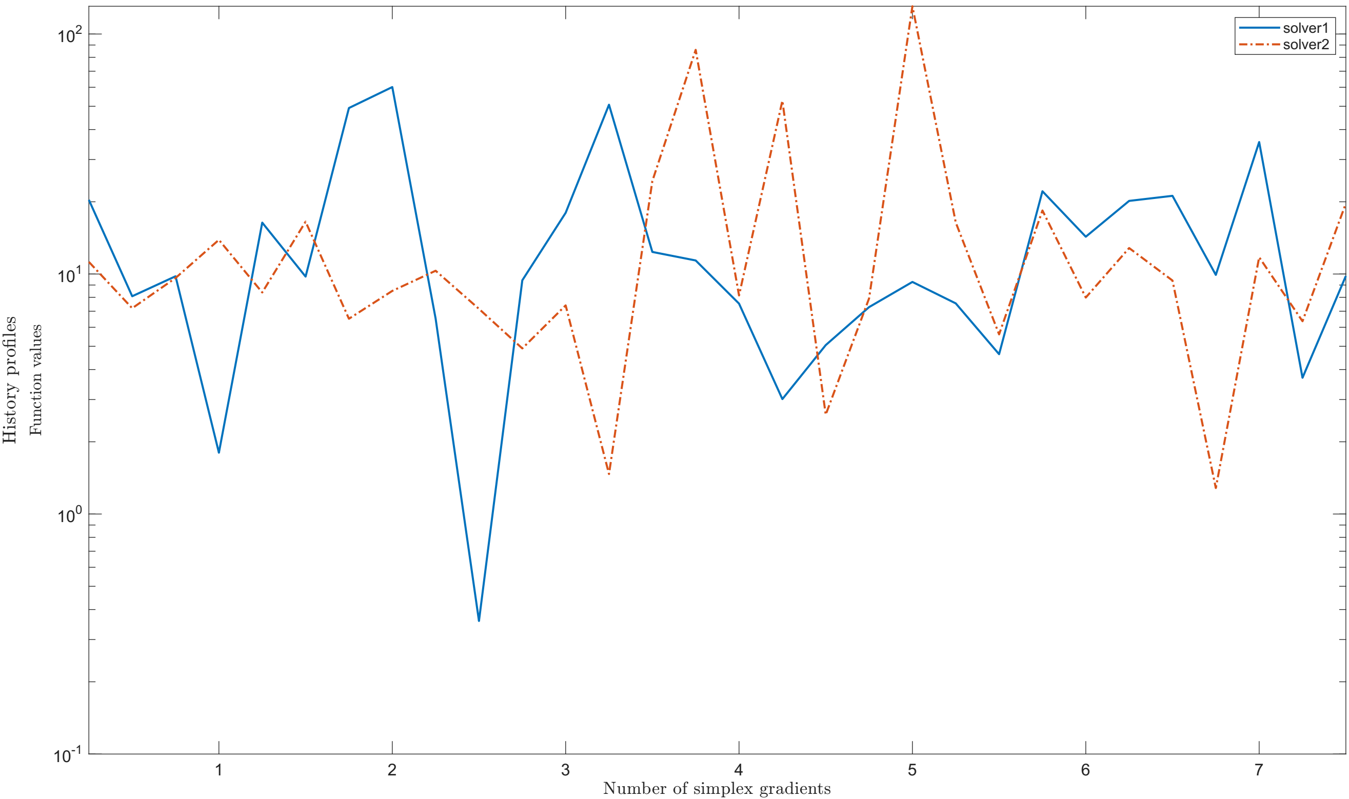
Solving “SSI” with “noisy_0.001_mixed_gaussian” feature
