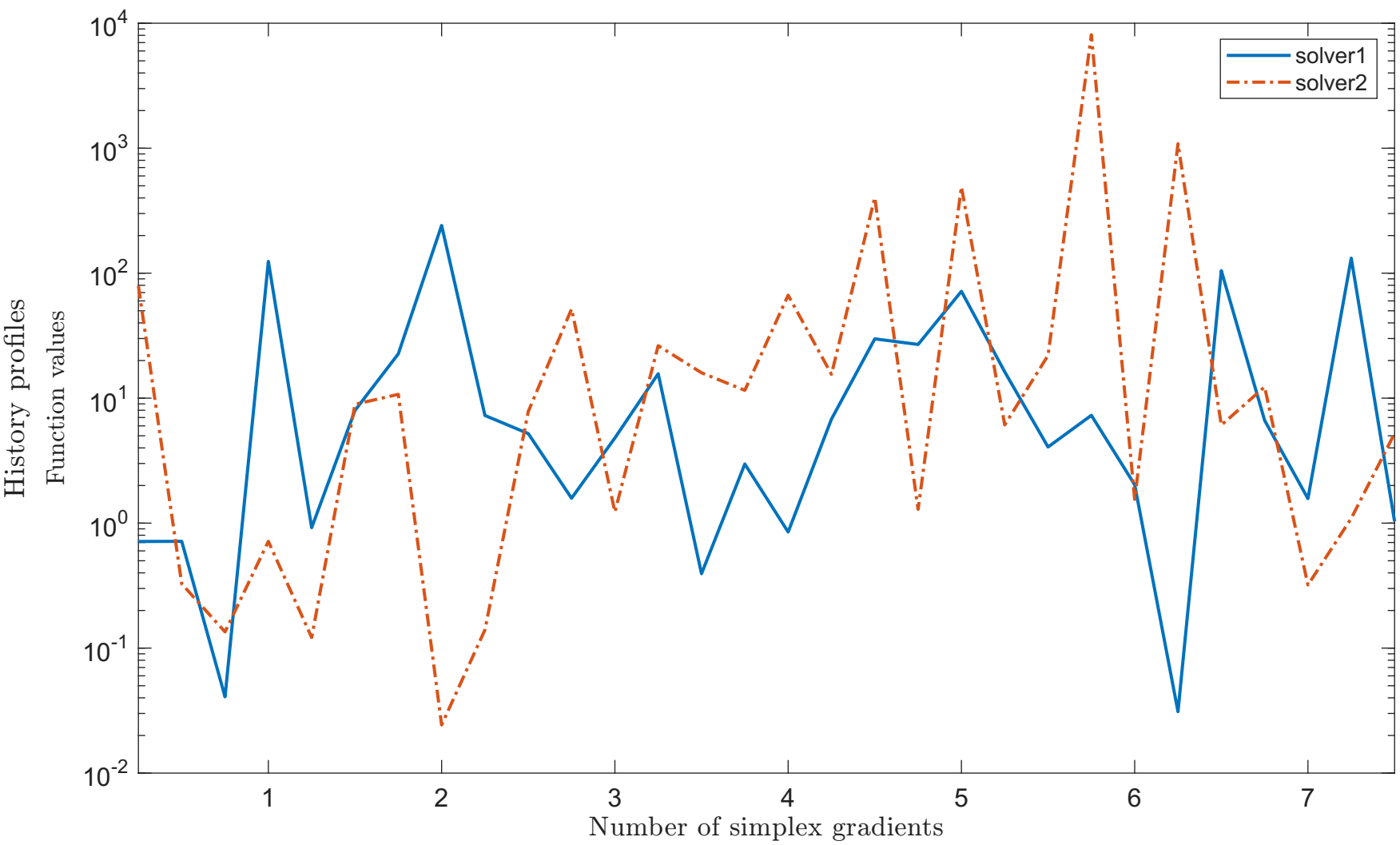
Solving “HATFLDFL” with “noisy_0.001_mixed_gaussian” feature
