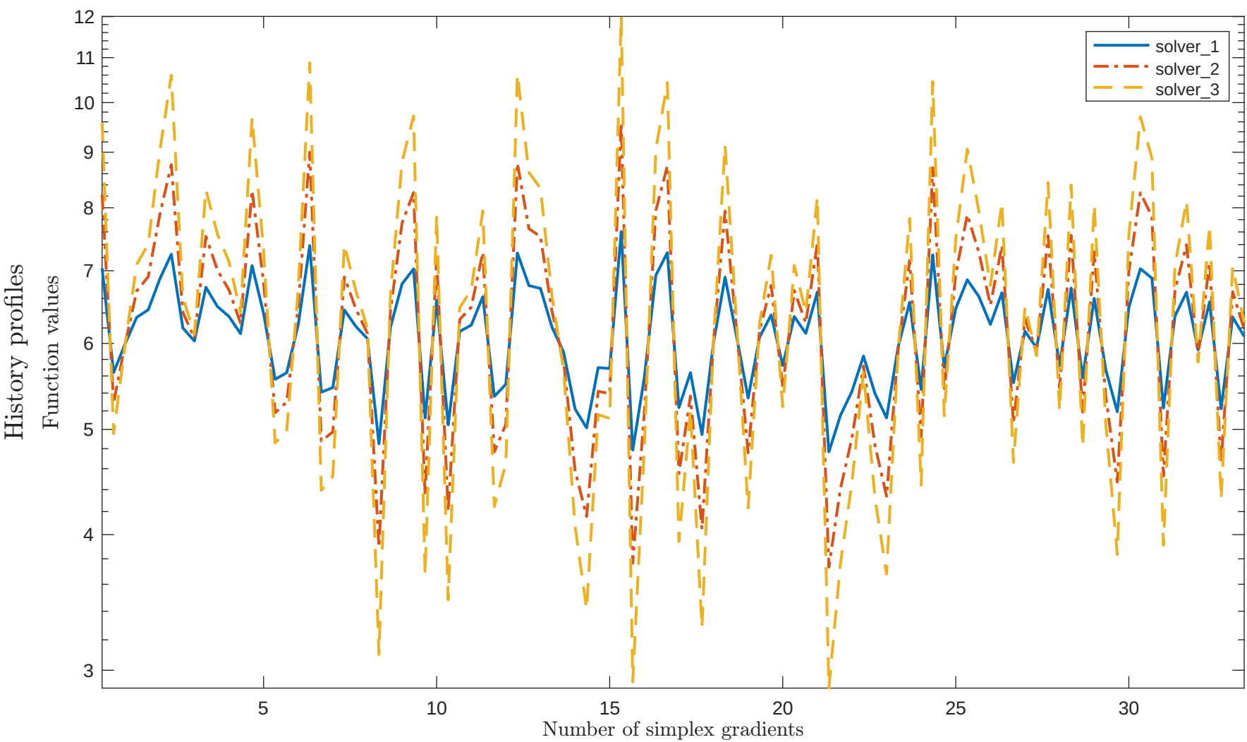
Solving “DENSCHNB” with “plain” feature
