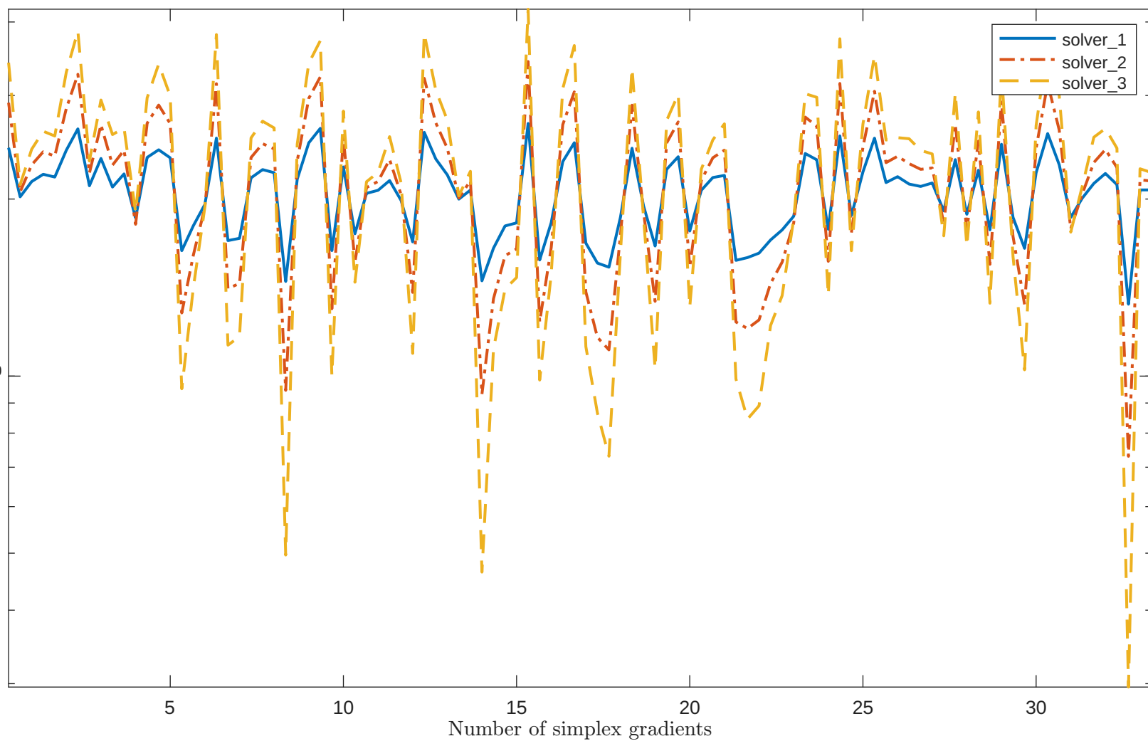
Solving "HIMMELBH" with "plain" feature
