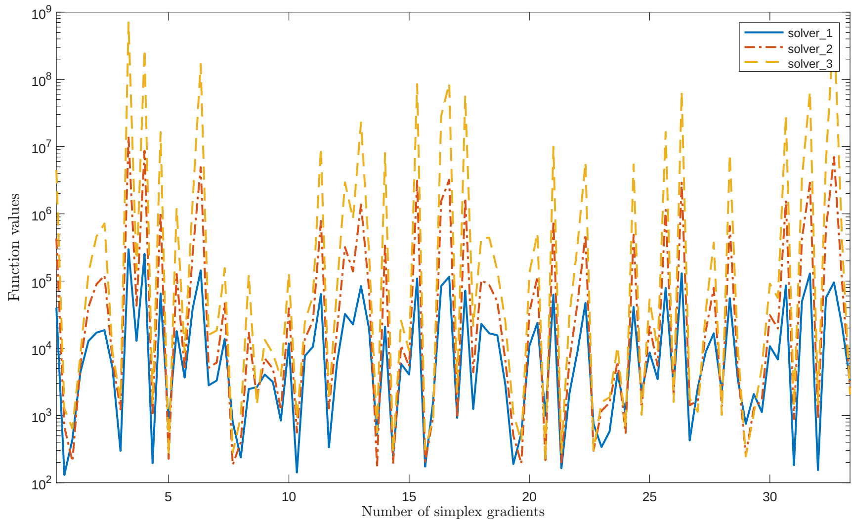
Solving “JENSMP” with “plain” feature
