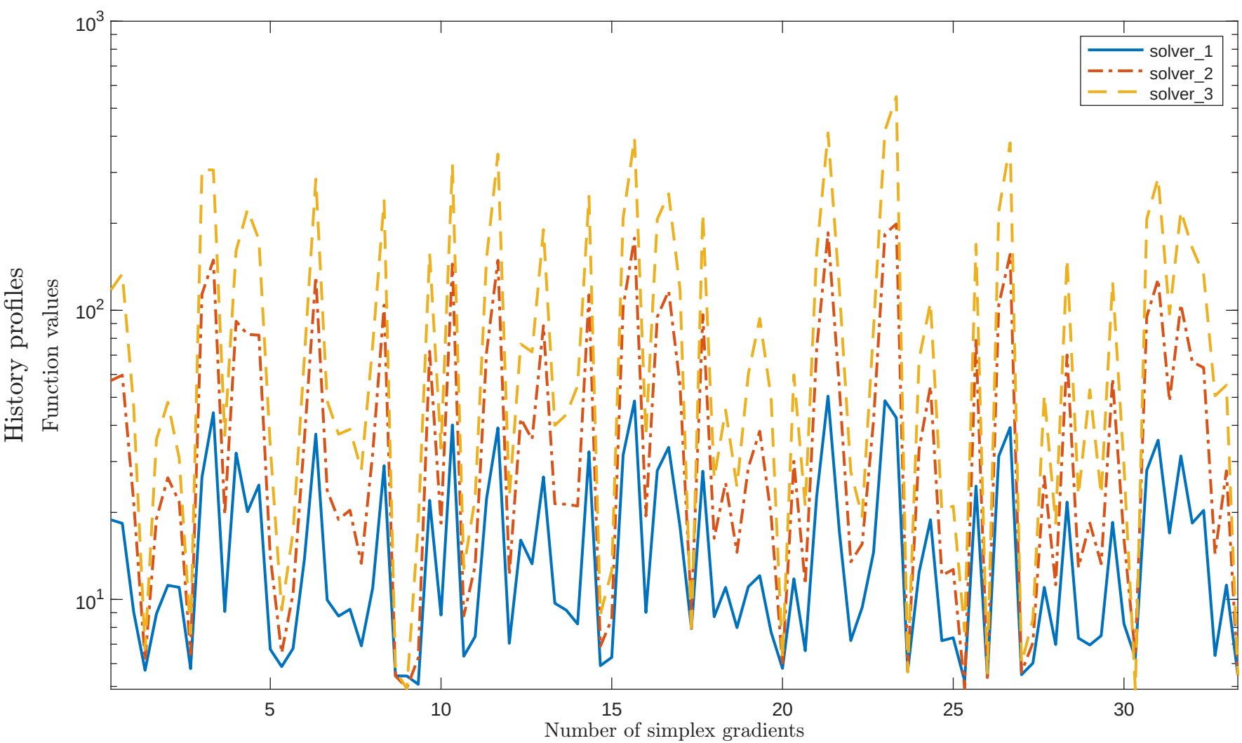
Solving "SINEVAL" with "plain" feature
