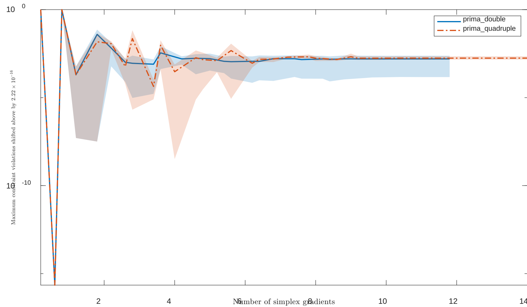
Solving "ALLINITC" with "noisy" feature
