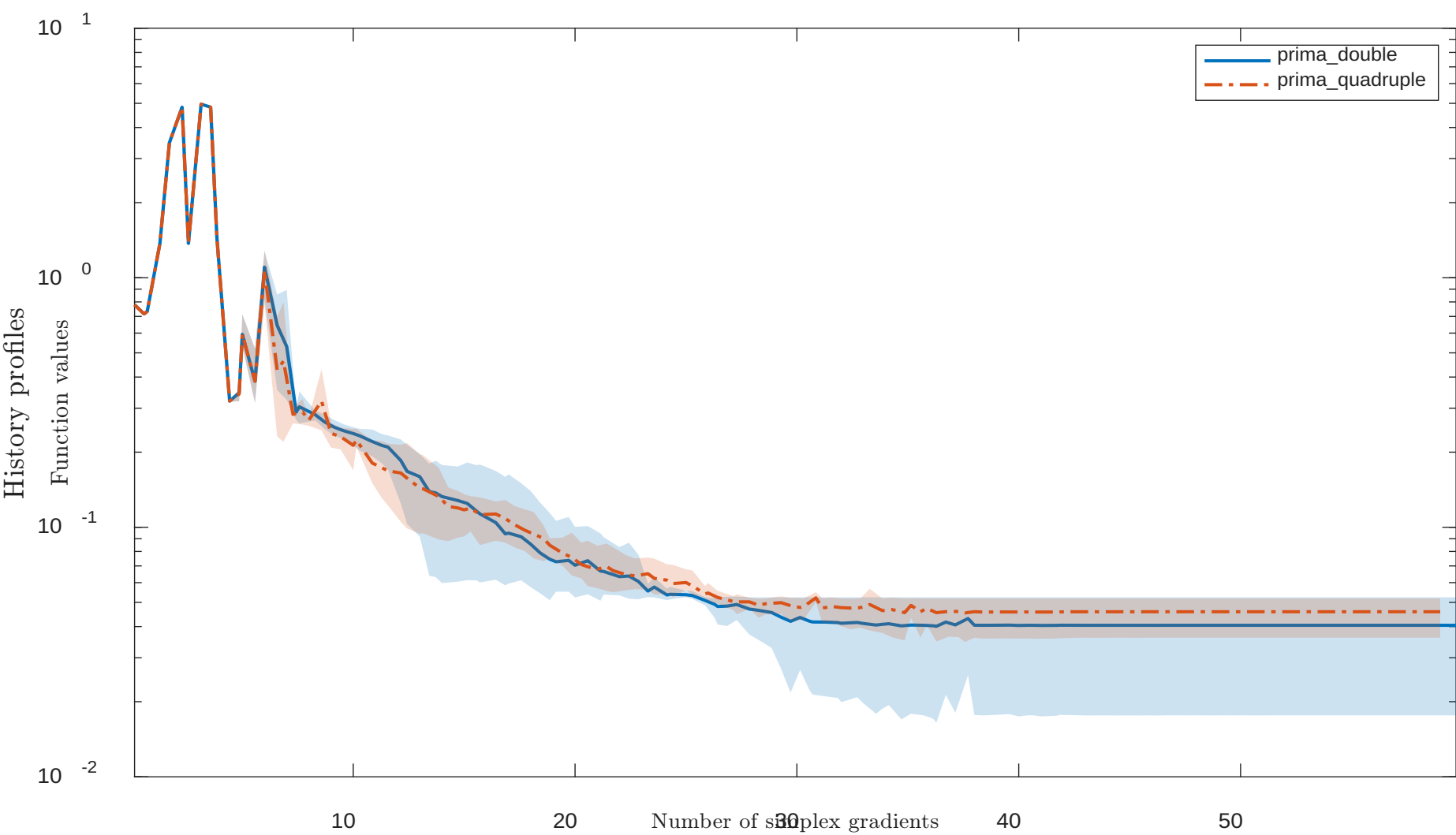
Solving “BIGGS6” with “noisy” feature
