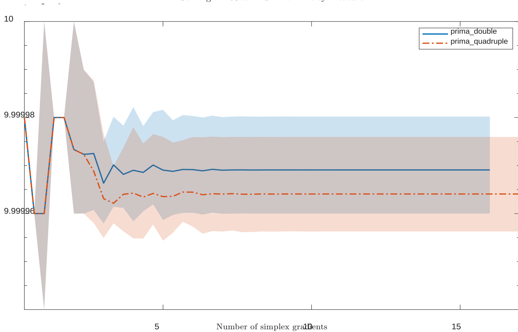
Solving “BROWNBS” with “noisy” feature
