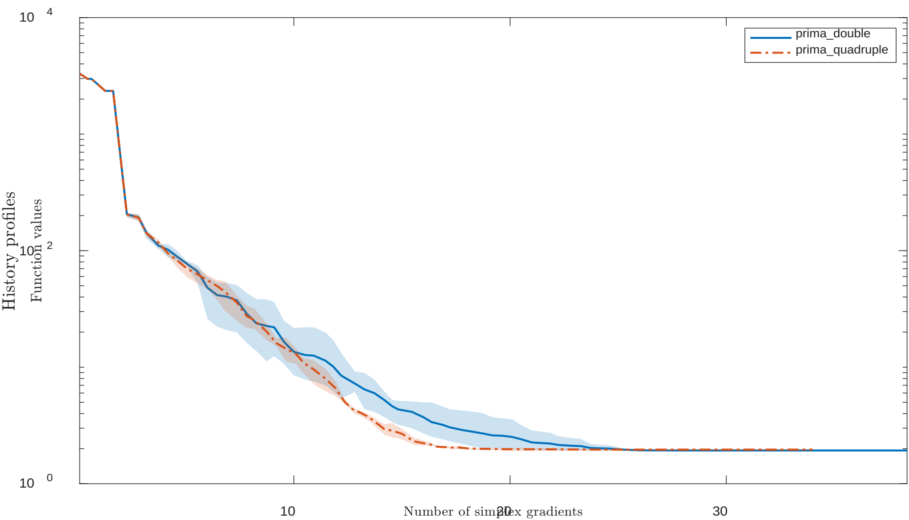
Solving “CRAGGLVY” with “noisy” feature
